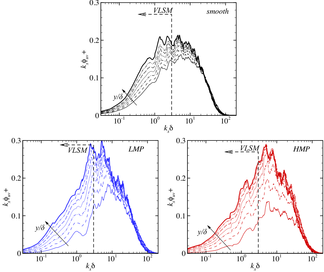
Figure 11. Premultiplied co-spectra, k_x \phi_{uv}^+ , as a function of streetwise wavelength, k_x \delta , for (a) smooth-wall flow and rough-wall flow along an (b) LMP and an (c) HMP. Dash vertical line demarcates the VLSM boundary ( k_x \delta < 2 ). For line legend, see figure 8.
