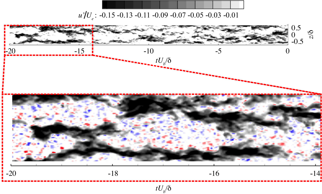
Figure 5. Wall-parallel ( x - z ) view of an LMR at y/\delta = 0.15 demarcated with contours of negative streamwise velocity fluctuation from Taylor’s hypothesis reconstruction. A zoomed-in region is also presented with color contours of signed swirling strength demarcating the locations of wall-normal vortex cores.
