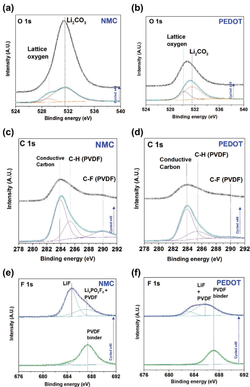
Figure 4. a,b) XPS spectra for O 1s of the cycled bare \text{Li}(\text{Ni}_{1/3}\text{Mn}_{1/3}\text{Co}_{1/3})\text{O}_2 (labeled as NMC) and PEDOT:PSS coated \text{Li}(\text{Ni}_{1/3}\text{Mn}_{1/3}\text{Co}_{1/3})\text{O}_2 cathode (labeled as PEDOT). c,d) C 1s of the cycled NMC cathode and PEDOT cathode. e,f) F 1s of the cycled NMC cathode and PEDOT cathode.
