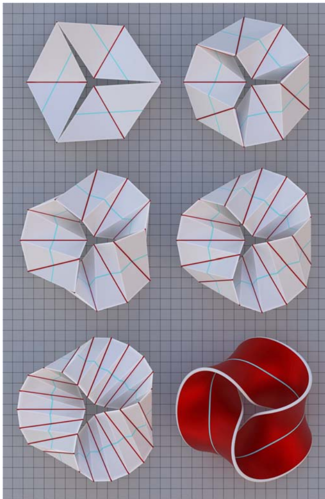
Fig. 10. The six-hinged kaleidocycle (K6) and a sequence of Möbius kaleidocycles MKN with increasing number N > 7 of minimally twisted tetrahedra together with the smooth limit surface \mathcal{S} illustrate the limit process N \rightarrow \infty . Shown are a K6 (Top Left), MK9 (Top Right), MK12 (Middle Left), MK15 (Middle Right), MK21 (Bottom Left), and the limit surface \mathcal{S} for N \rightarrow \infty (Bottom Right), a 3\pi -twist Möbius band. The hinges are red, and the limit surface, viewed as a collection of infinitely many hinges, is also red. Note that threefold symmetric rings are chosen only for aesthetic reasons; the limit sequence consists of all natural numbers N \geq 6 .
