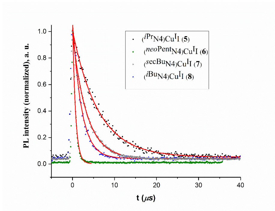
Figure 12. Normalized Photoluminescence decay profiles for CuI complexes 5-8 (500-800 nm range) in \text{CH}_2\text{Cl}_2 solution at 298 K. Excitation at 400 nm.
