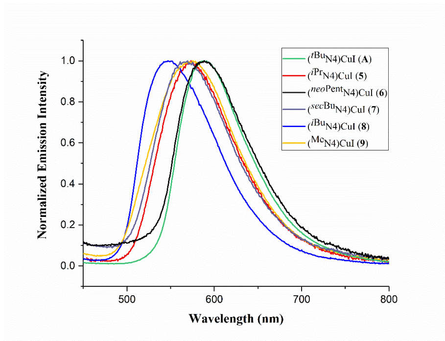
Figure 9. Normalized emission spectra of complexes t\text{BuN}_4\text{CuI} (A), i\text{PrN}_4\text{CuI} (5), neo\text{PentN}_4\text{CuI} (6), sec\text{BuN}_4\text{CuI} (7), i\text{BuN}_4\text{CuI} (8) and \text{MeN}_4\text{CuI} (9) in the solid state at 298 K; excitation at 400 nm.
