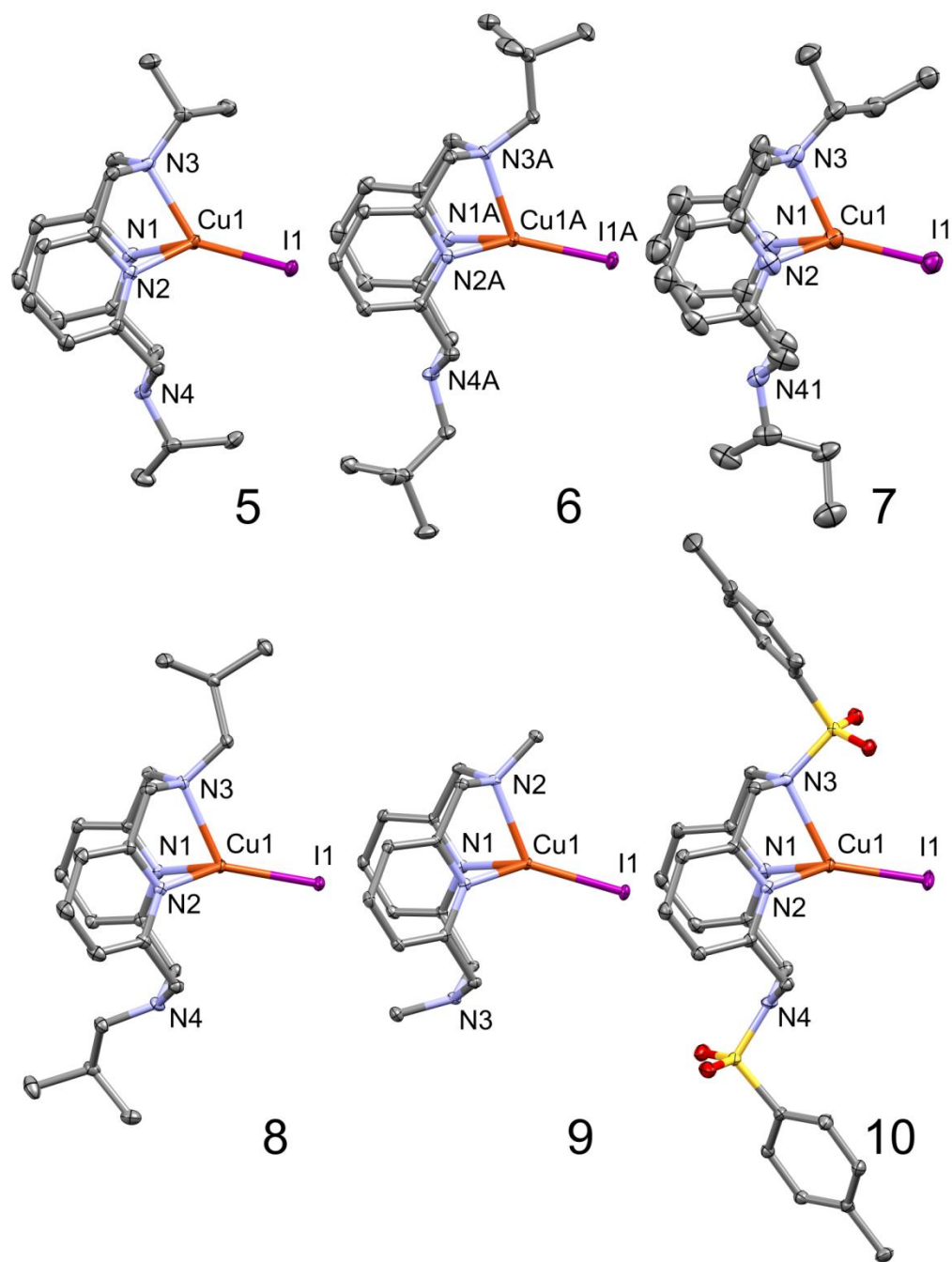
Figure 2. ORTEP projections of iodide complexes (^R\text{N}4)\text{CuI} 5-10 showing anisotropic displacement ellipsoids at 50% probability level if not indicated otherwise. For complex 6 , only one independent molecule A is shown. For complex 7 , displacement ellipsoids are shown at 30% probability level for clarity. Hydrogen atoms, minor components of disorder and a solvent molecule in the case of (^T\text{S}\text{N}4)\text{CuI} 10 are omitted for clarity.
