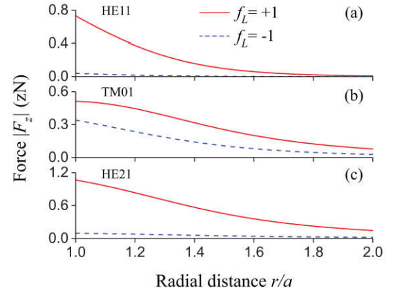
FIG. 2. Radial dependence of the absolute value |F_z| of the axial component of the force of the resonant guided light on a two-level atom. The incident light field is in (a) an x -polarized HE 11 mode, (b) a TM 01 mode, or (c) an x -polarized HE 21 mode and propagates in the forward f_L = + (solid red curves) or backward f_L = - (dashed blue curves) direction along the fiber axis z with the power P = 1 pW. The dipole matrix element of the atom is \mathbf{d}_{eg} = d(i\hat{x} - \hat{z})/\sqrt{2} , the fiber radius is a = 350 nm, and the wavelength of the atomic transition is \lambda_0 = 780 nm. The refractive indices of the fiber and the vacuum cladding are n_1 = 1.4537 and n_2 = 1 , respectively.
