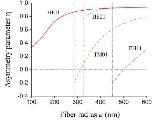
FIG. 5. Asymmetry parameter \eta for the axial forces F_z^{(f_L)} for the opposite propagation directions f_L = \pm as a function of the fiber radius a . The parameters used are the same as for Fig. 4. The vertical dotted lines indicate the positions of the cutoffs for higher-order modes.
