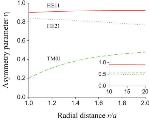
FIG. 3. Radial dependence of the asymmetry parameter \eta for the axial forces F_z^{(f_L)} for the opposite propagation directions f_L = \pm . The parameters used are the same as for Fig. 2. The inset shows the parameter \eta in the limit of large distances r .
