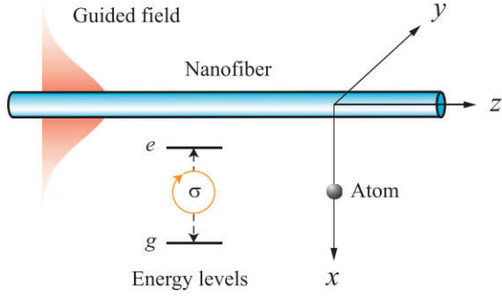
FIG. 1. Two-level atom with a dipole rotating in the meridional plane zx outside an ultrathin optical fiber.
