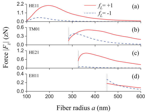
FIG. 4. Absolute value |F_z| of the axial component of the force of the resonant guided light on a two-level atom as a function of the fiber radius a . The atom is positioned at the distance r - a = 20 nm from the fiber surface. Other parameters are as for Fig. 2. The vertical dotted lines indicate the positions of the cutoffs for higher-order modes.
