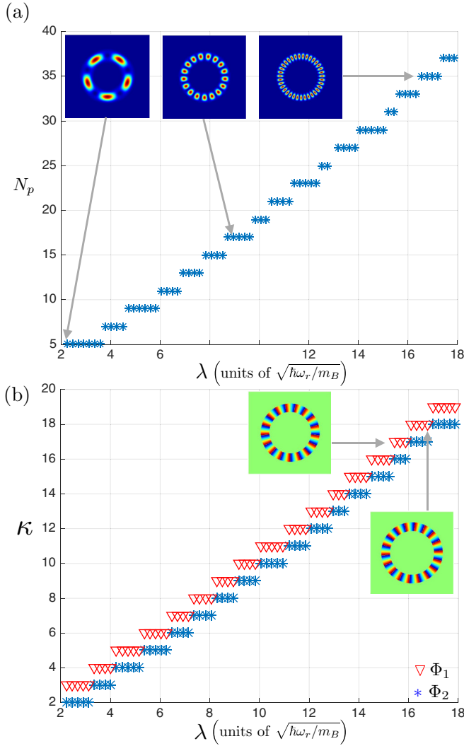
FIG. 2. (a) Number of petals as a function of the spin-orbit-coupling strength in the immiscible regime g_{12}/g = 1.6 . The insets show the density profiles of a single component, confirming the typical necklacelike appearance over a large range of values of \lambda . (b) Winding numbers of \Phi_1 and \Phi_2 as a function of the spin-orbit-coupling strength \lambda in the miscible regime ( g_{12}/g = 0.6 ). The insets show the phase profile for \lambda = 16.8 . Here r_0 = 1.12 .
