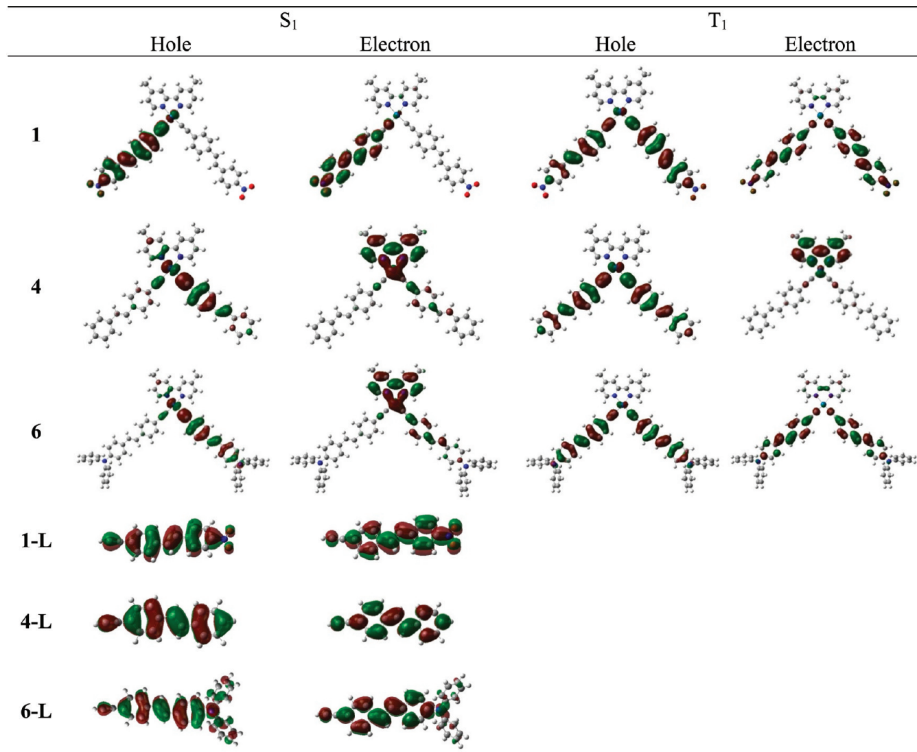
Figure 5. NTO plots for the singlet ( S_1 ) and triplet ( T_1 ) emissions (corresponding to the fluorescence and phosphorescence, respectively) for complexes 1, 4, and 6 and their corresponding ligands 1-L, 4-L, and 6-L. NTOs were obtained based on the optimized excited-state geometry to simulate the photoluminescence.
