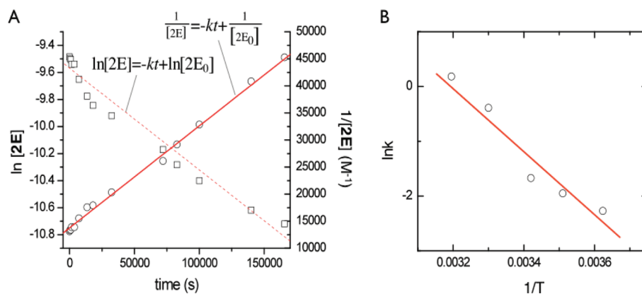
Figure 3. Kinetic studies on 2. (A) Kinetic analysis of the spectrophotometric data obtained at 292 K. (B) Arrhenius plot giving an E_a = 12100 \text{ cal mol}^{-1} .
