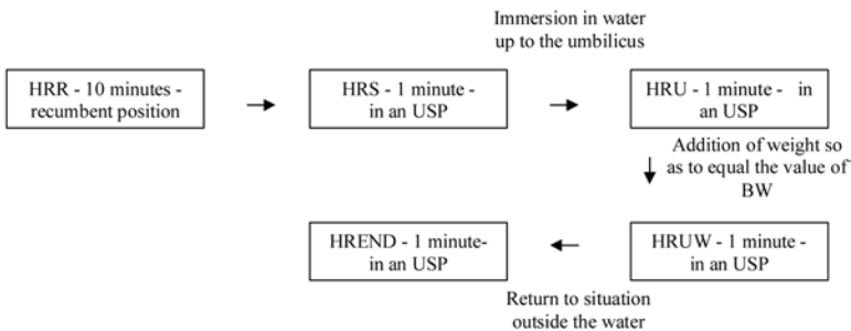
Figure 1 — Experiment’s protocol. Note. HRR, heart rate at rest; HRS, standing heart rate; HRU, immersion in water up to the umbilicus; HRUW, immersion in water up to the umbilicus with weight; HREND, heart rate end; BW, body weight; USP, upright standing position.
