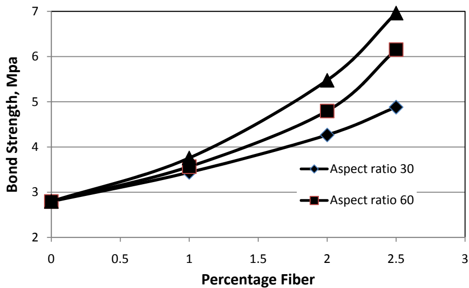
Figure 2: Effect of fiber content on bond strength
