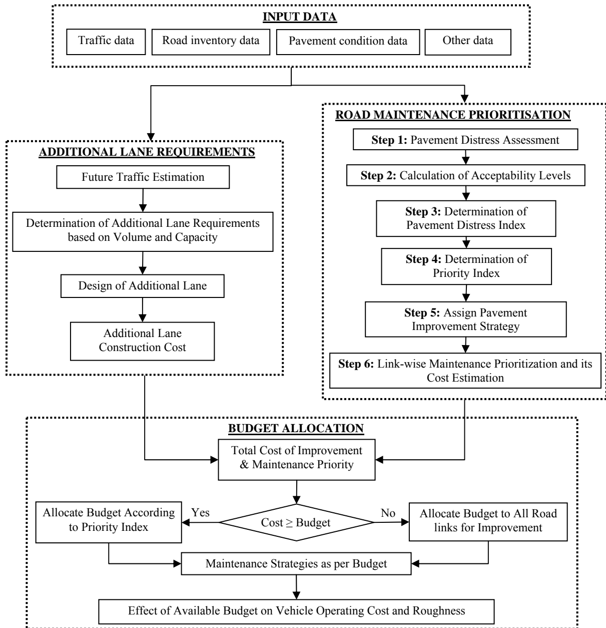
Figure 1: Description of Road Maintenance and Rehabilitation System
