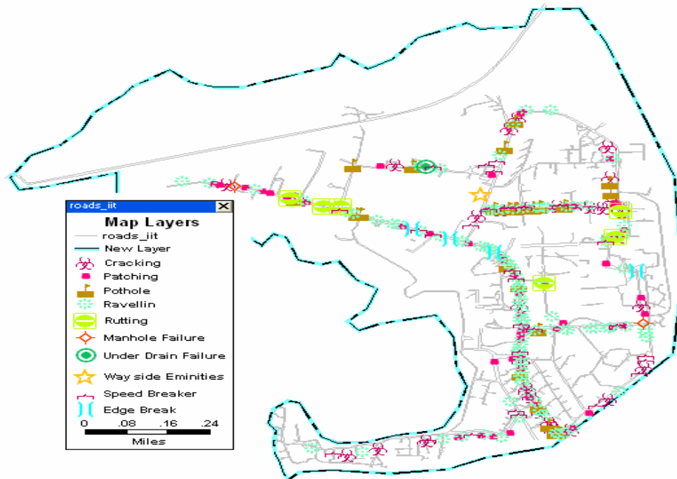
Figure 3: Pavement Condition Data
