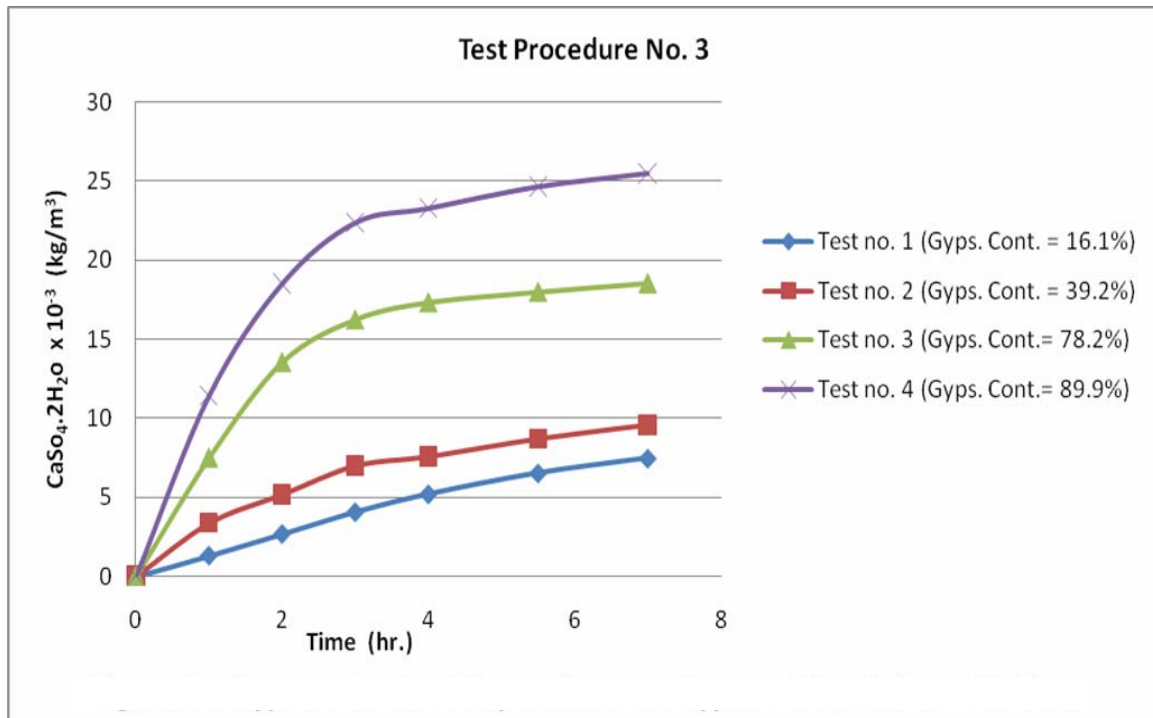
Figure 14: Gypsum content dependence on gypsum dissolution with time
