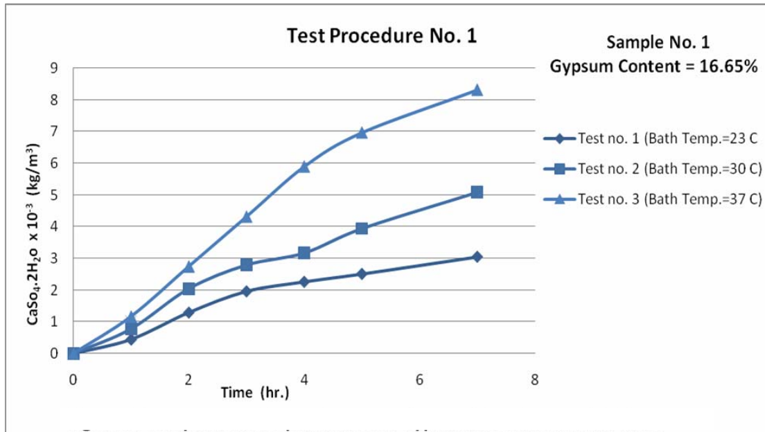
Figure 9: Temperature dependence on gypsum dissolution with time
