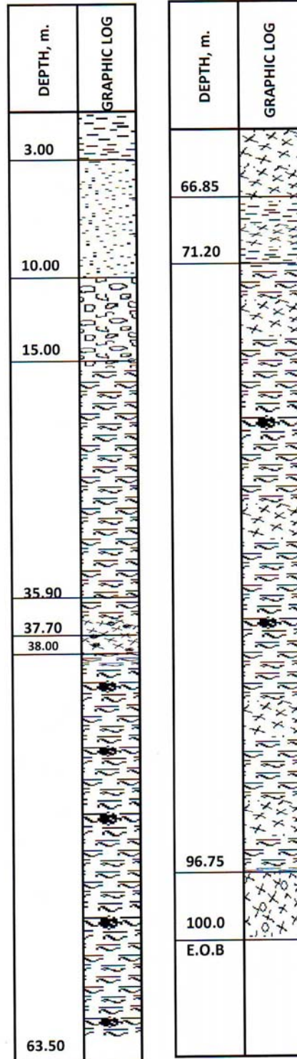
Figure 3: Layout for borehole 2
