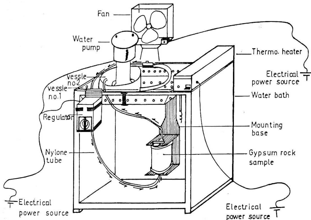
Figure 7: Layout of the setup
