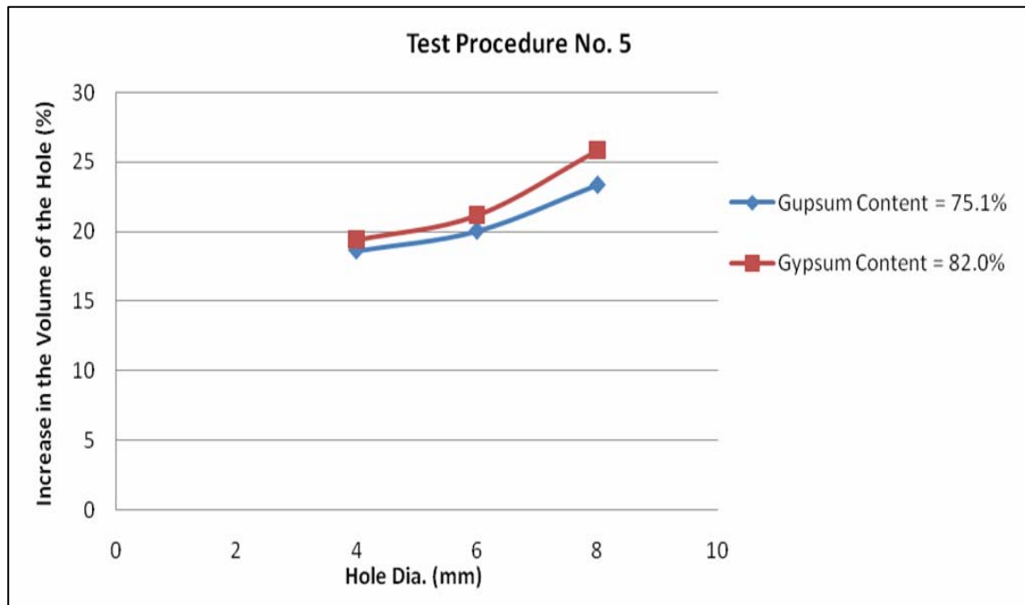
Figure 22: Increase in the volume of the hole vs. hole diameter
