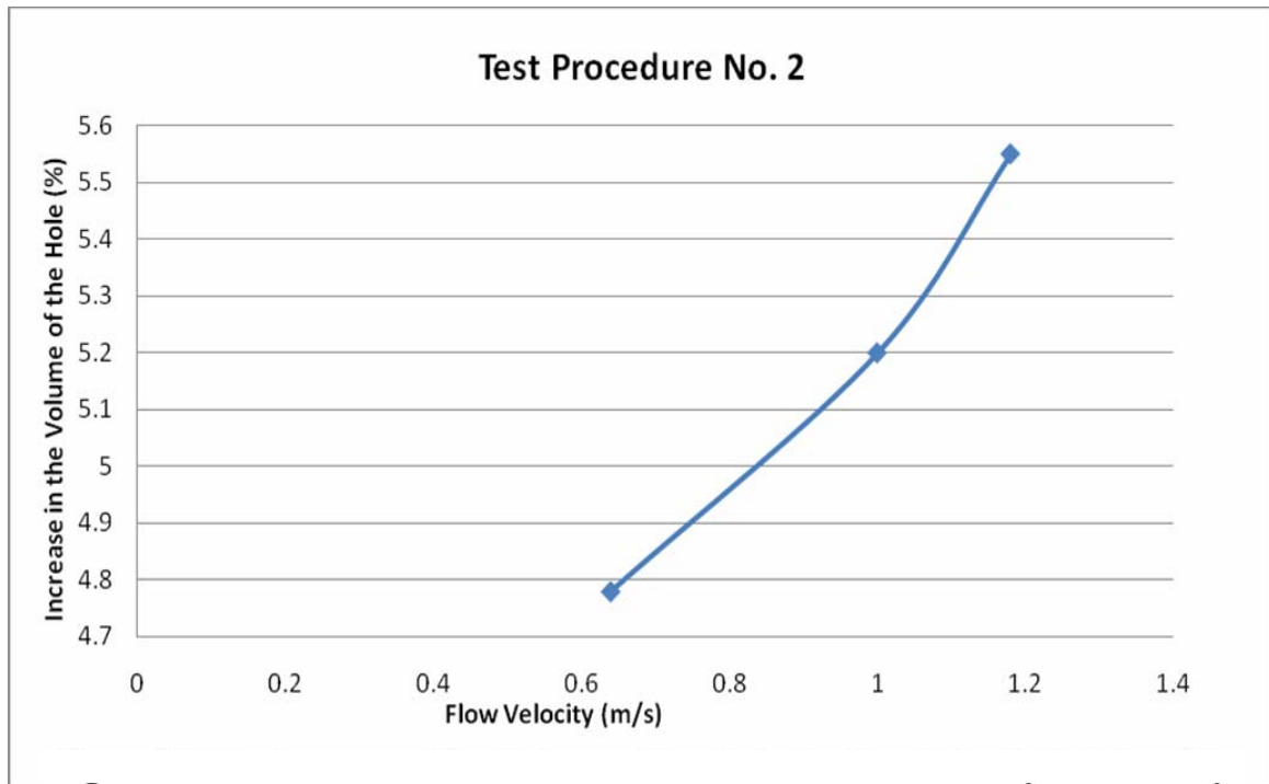
Figure 12: The increase in the volume of the hole vs. flow velocity relationship
