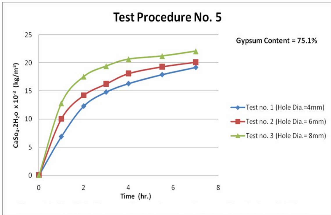
Figure 20: The hole diameter dependence on gypsum dissolution with time
