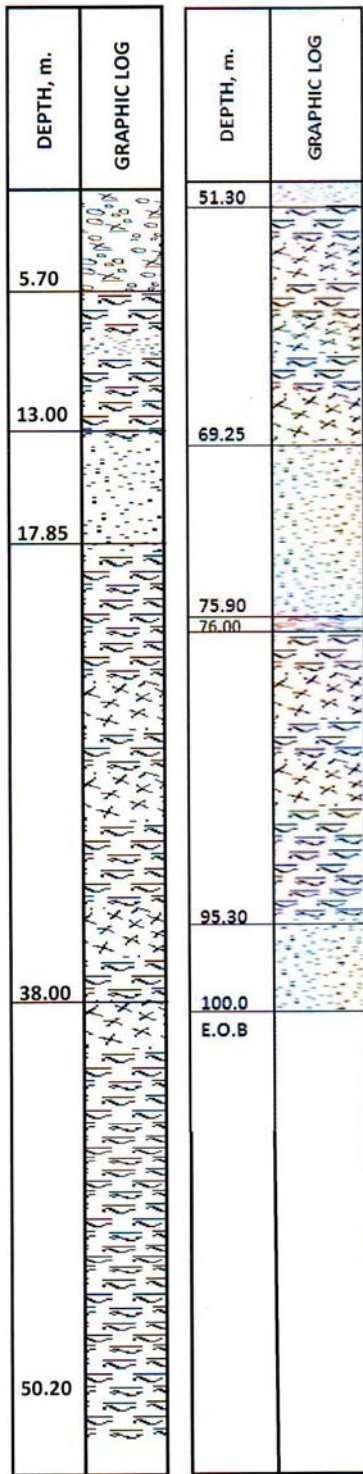
Figure 4: Layout for borehole 3
