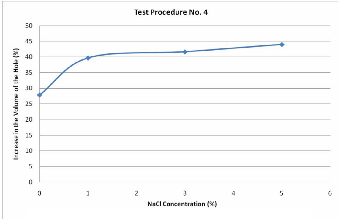
Figure 19: Increase in the volume of the hole vs. water salinity
