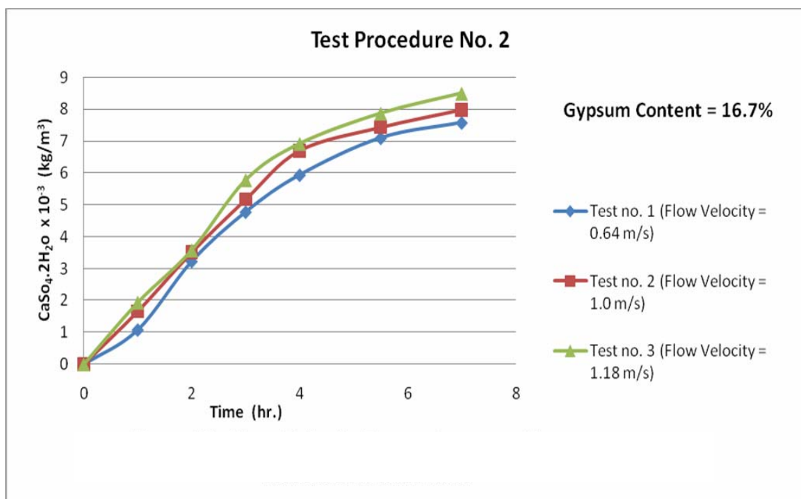
Figure 11: Flow velocity dependence on gypsum dissolution with time
