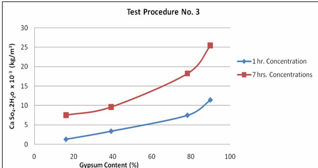
Figure 15: Effect of gypsum content on the amount and rate of gypsum dissolution
