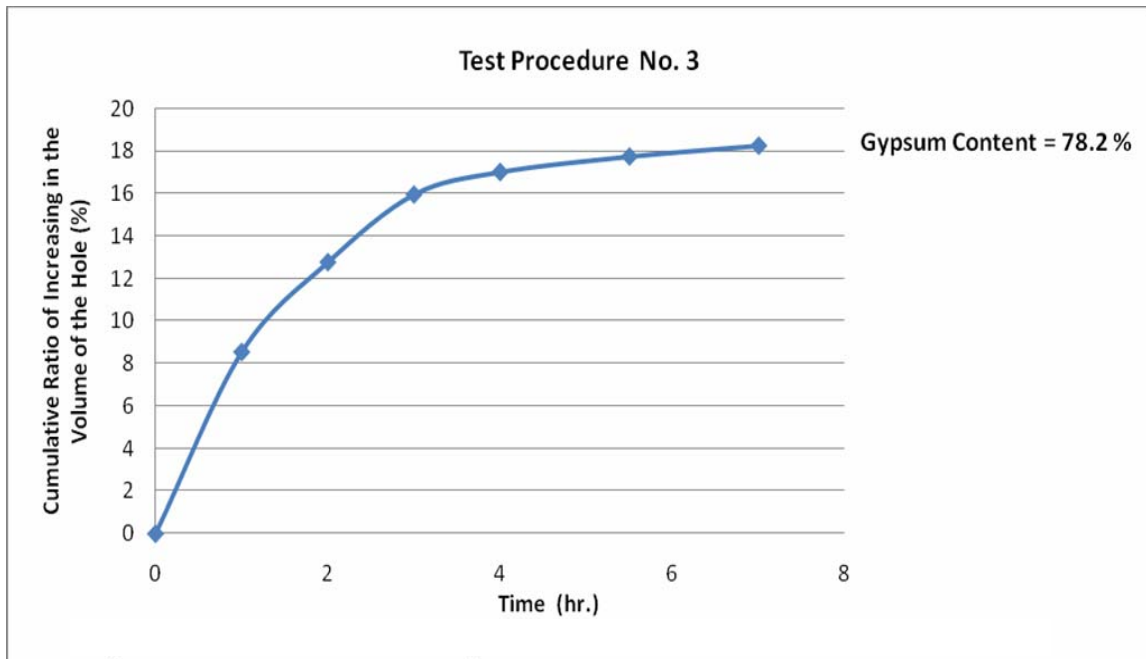
Figure 17: Ratio of increase in the volume of the axial hole vs. time
