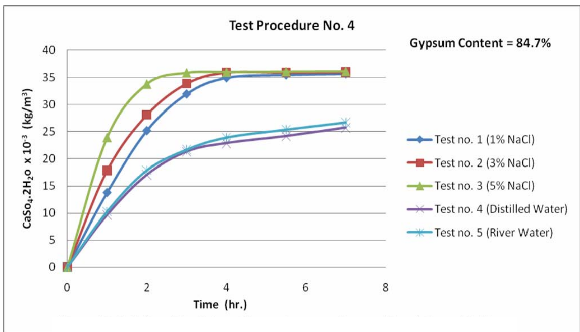
Figure 18: Salinity of the solvent dependence on gypsum dissolution with time
