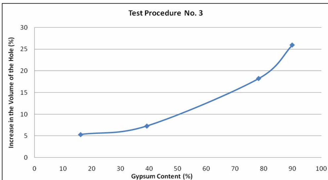
Figure 16: Increase in the volume of the hole vs. gypsum content relationship
