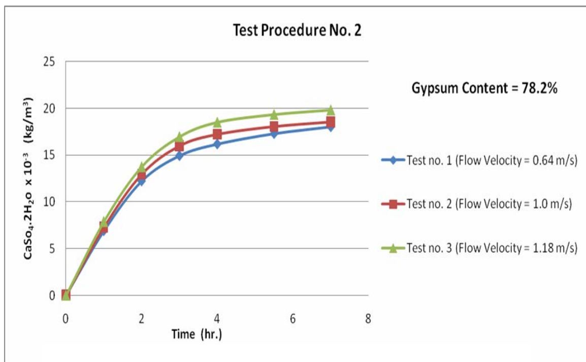
Figure 13: Flow velocity dependence on gypsum dissolution with time
