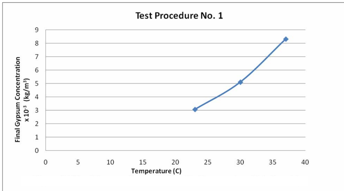
Figure 10: Final gypsum concentration vs. temperature relationship
