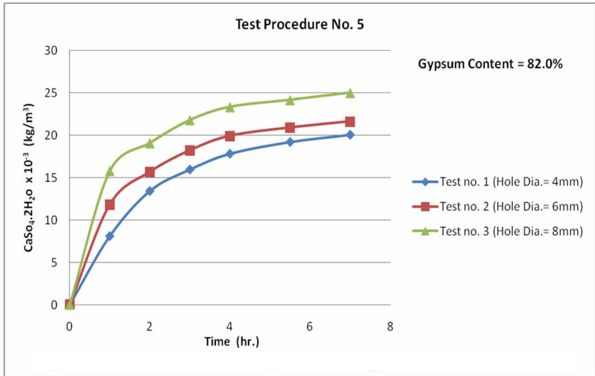
Figure 21: Axial hole diameter dependence on gypsum dissolution with time
