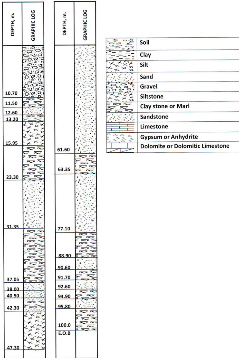
Figure 6: Layout for borehole 5
