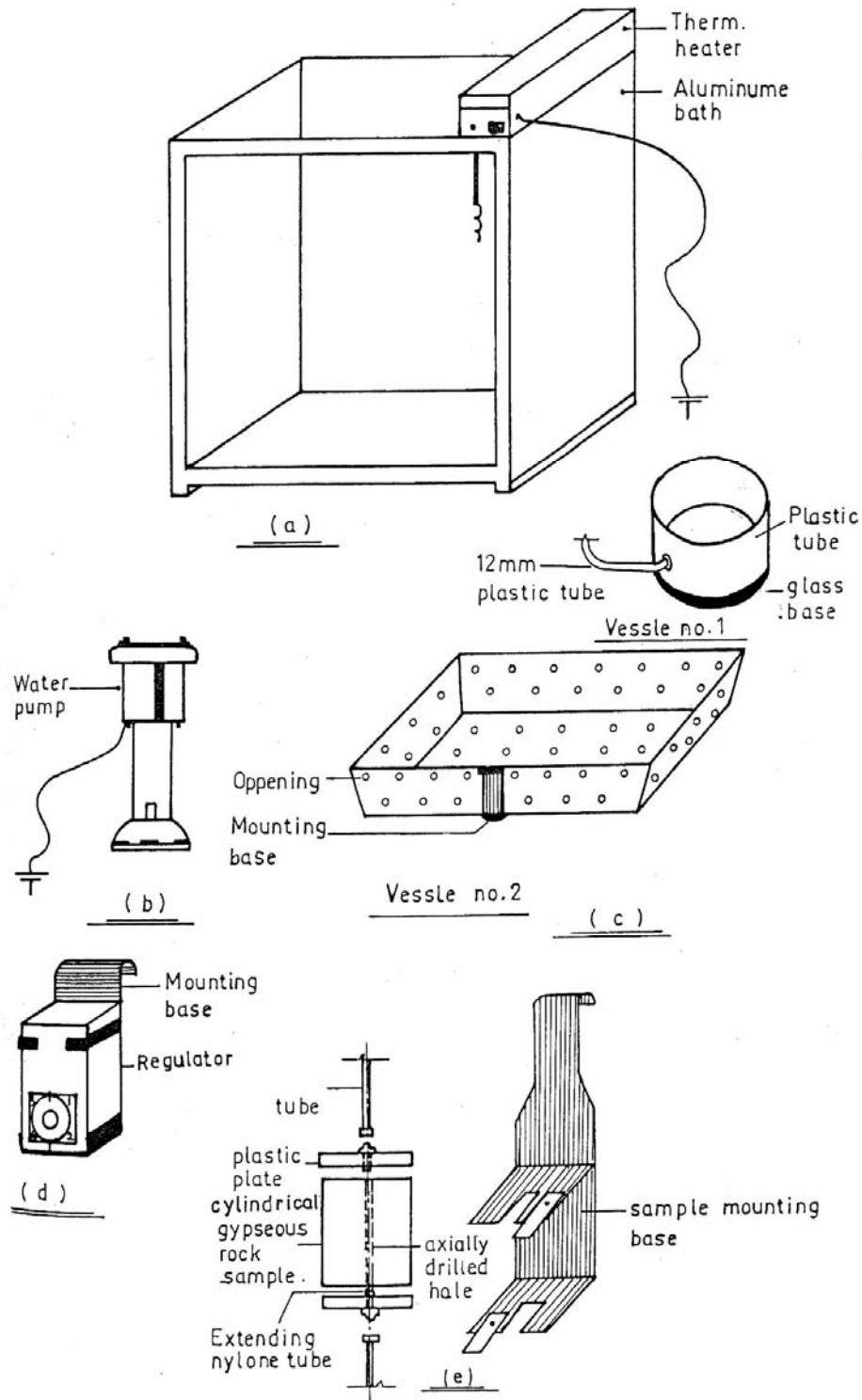
Figure 8: Details of the experimental setup
