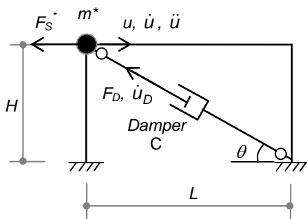
Figure 2: Lumped mass as GSDOF
