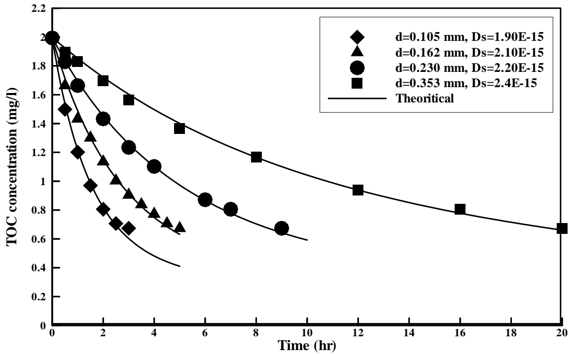
Figure (2): Batch reactor NOM adsorption onto GAC for various GAC particle sizes.
