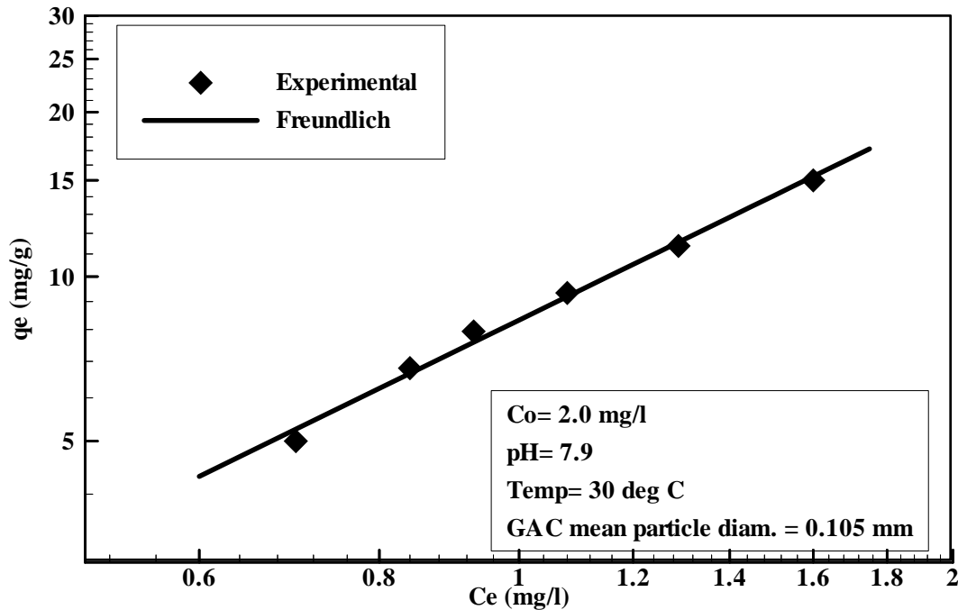
Figure (1): Raw water NOM adsorption equilibrium isotherm.
