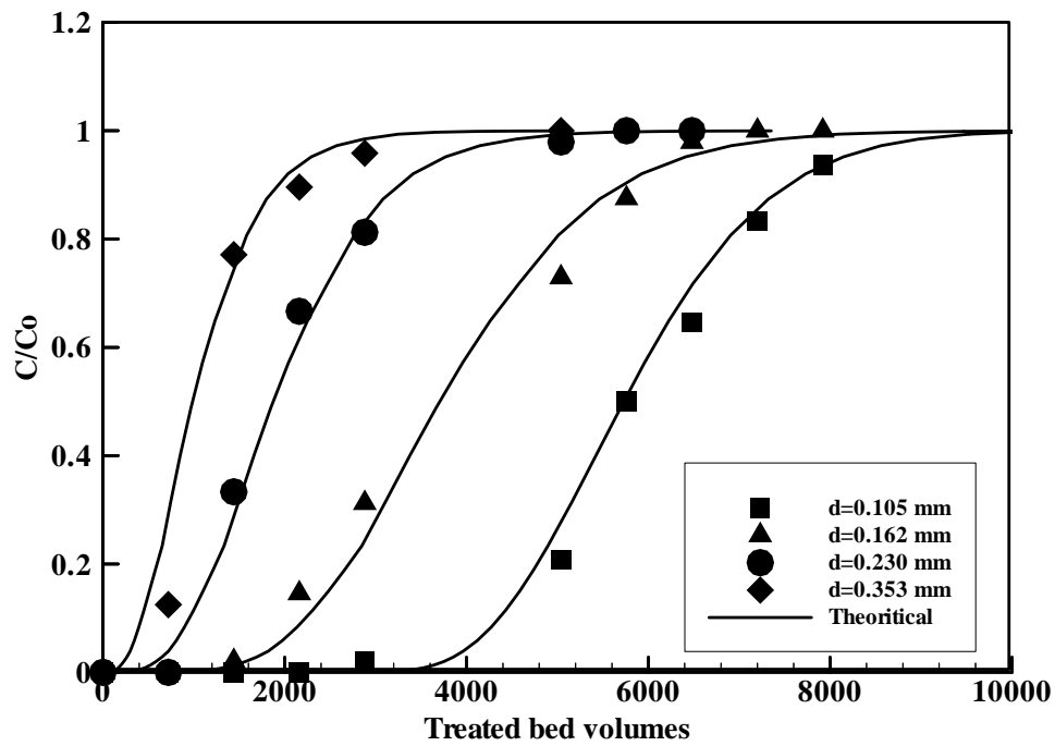
Figure (4): RSSCT experimental results and predictive fixed bed mathematical model results for different GAC mean particle sizes.
