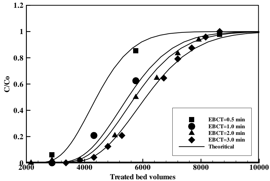
Figure (3): RSSCT experimental results and predictive fixed bed mathematical model results for different EBCTs.
