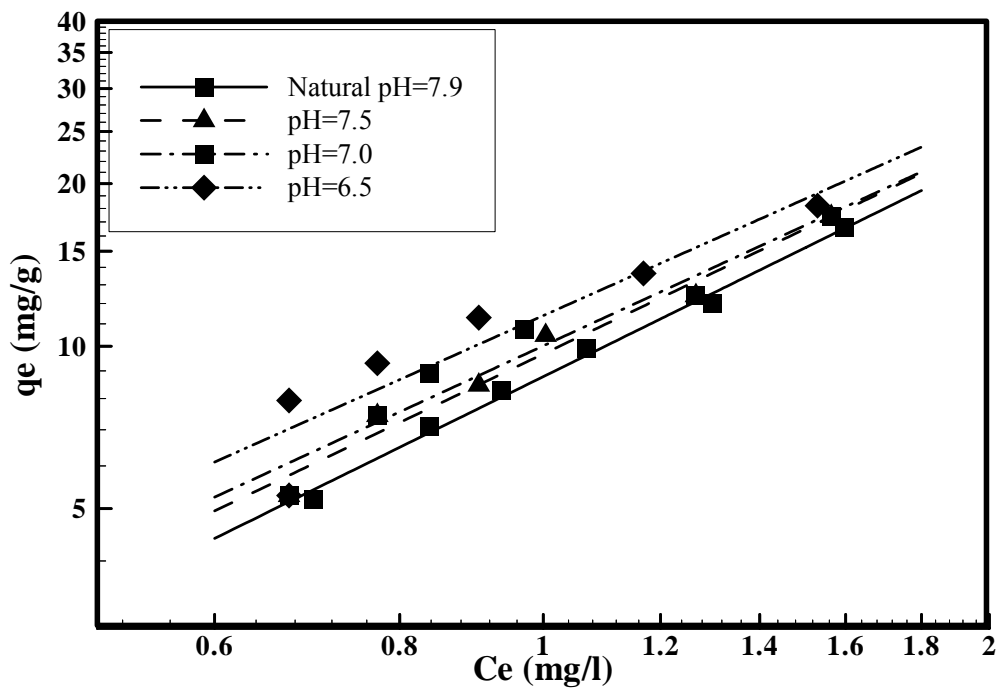
Figure (5): Effect of raw water pH on the adsorption equilibrium isotherm.
