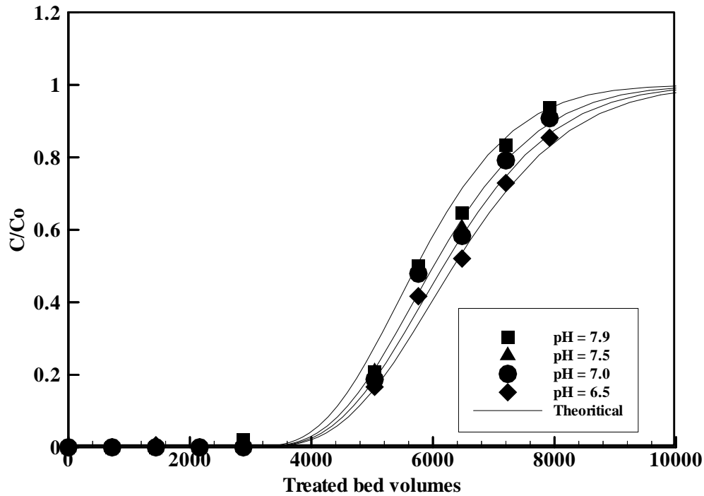
Figure (6): Effect of raw water pH on the behavior of RSSCT breakthrough curves.
