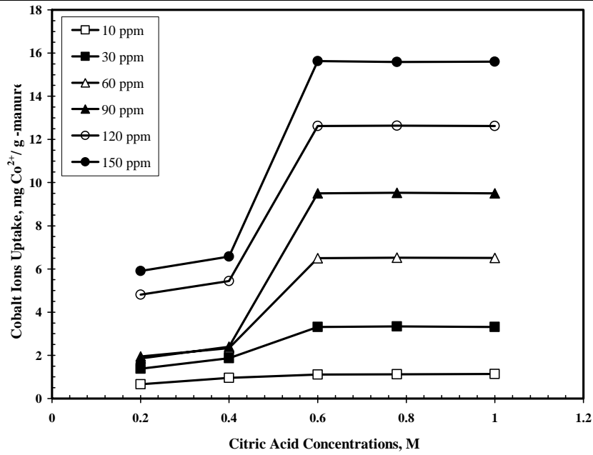
Figure (1): Effect of citric acid concentrations on cobalt ions uptake for C-SM when initial cobalt ions concentrations vary from 10 to 150 ppm, adsorbent concentration = 8 mg/ml, agitation time of 1 hr and solution pH = 6.
