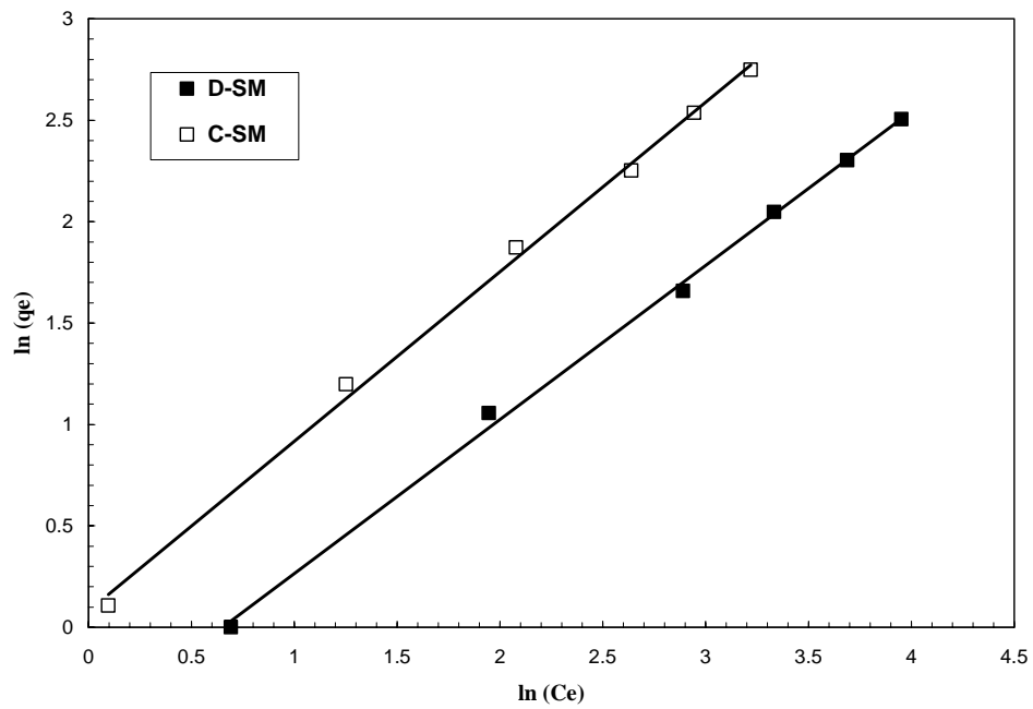
Figure (7): Freundlich isotherms for D-SM and C-SM.
