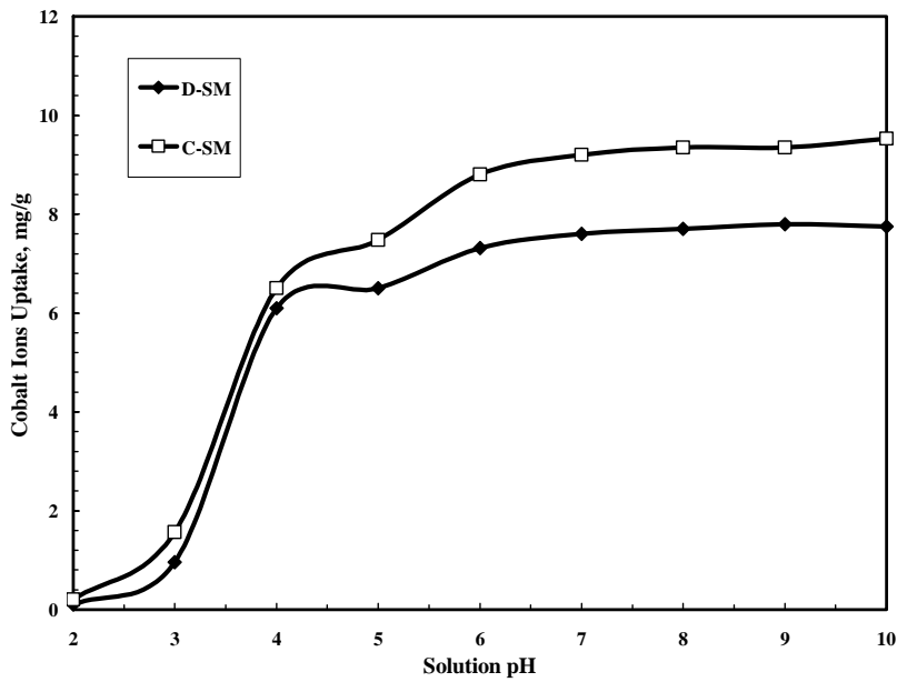
Figure (4): Effect of solution pH on cobalt ions uptake for D-SM and C-SM adsorbent concentration = 8 mg/ml, agitation time of 1 hr and initial cobalt ions concentration of 80 ppm.
