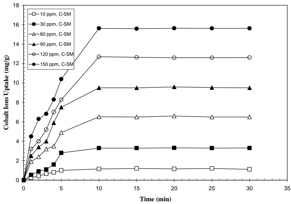
Figure (3): Effect of contact time and initial cobalt ions concentration on cobalt ions uptake for C-SM at solution pH = 6 and adsorbent concentration = 8 mg/ml.
