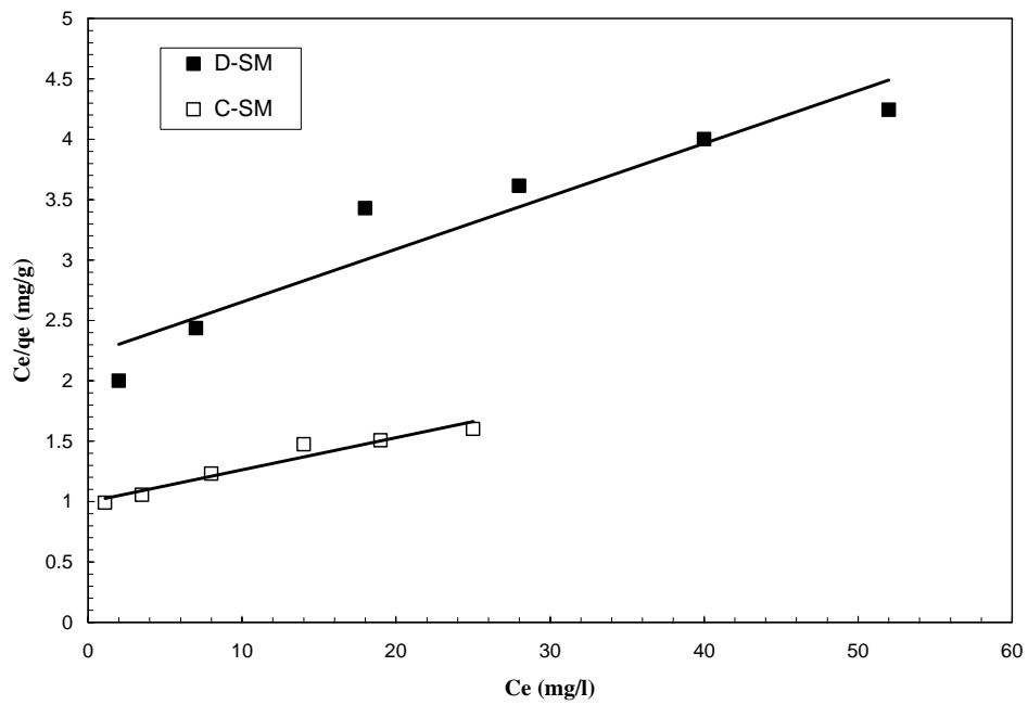
Figure (6): Langmuir isotherms for D-SM and C-SM.
