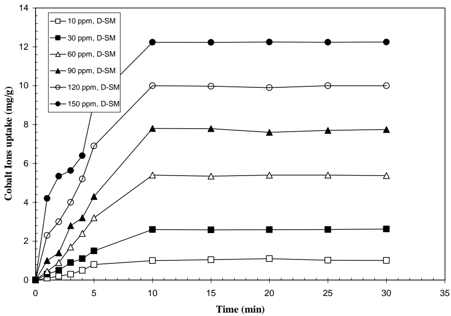
Figure (2): Effect of contact time and initial cobalt ions concentration on cobalt ions uptake for D-SM at solution pH=6 and adsorbent concentration =8 mg/ml.
