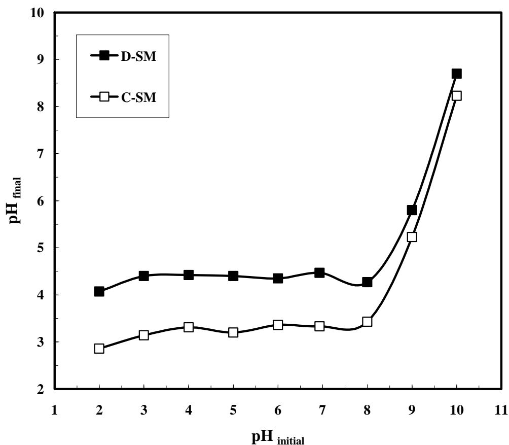
Figure (5): Point of zero charge for D-SM and C-SM.
