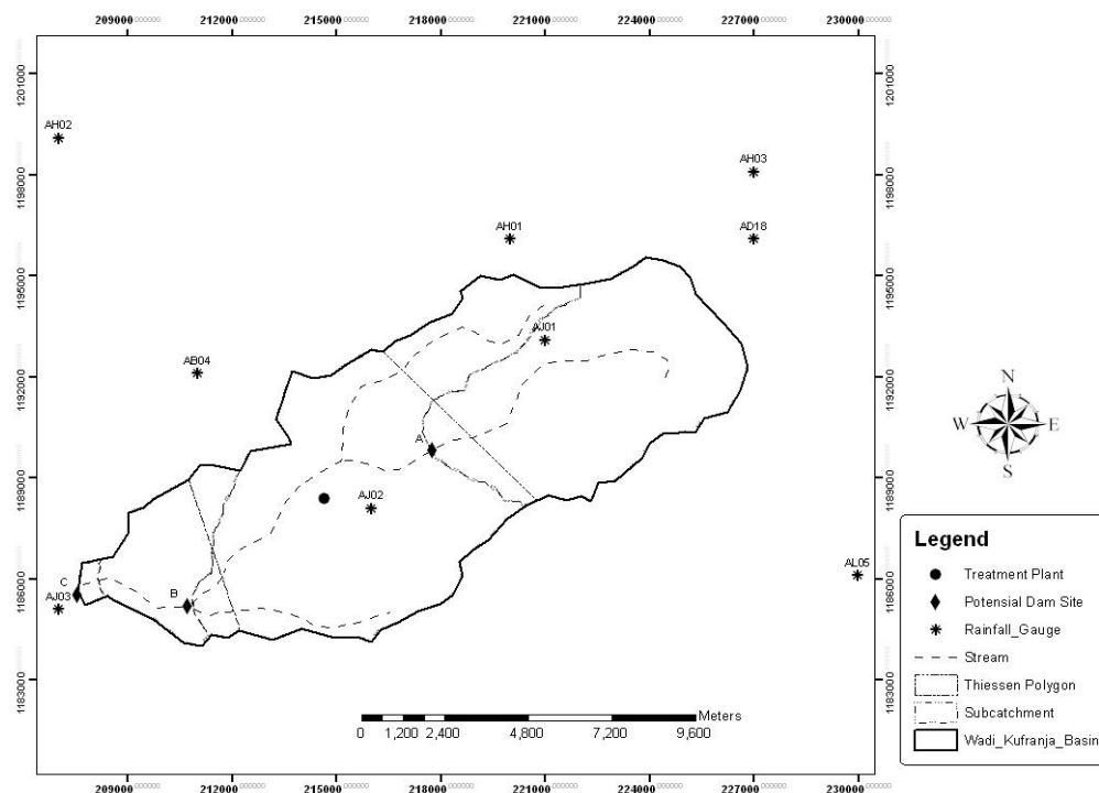
Figure 1: Kufranja Basin.
