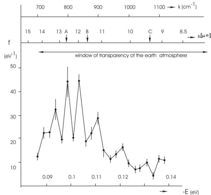
Figure 5. NES-spectrum of deionized water (chemical purity – 99.99 %; pH – 6.5–7.5; total mineralization – 200 mg/l; electric conductivity – 10 \mu\text{S/cm} ). The horizontal axis shows the energy of the H...O hydrogen bonds in the associates – E (eV). The vertical axis – energy distribution function – f ( \text{eV}^{-1} ). k – the vibration frequency of the H–O–H atoms ( \text{cm}^{-1} ); \lambda – wavelength ( \mu\text{m} ).
