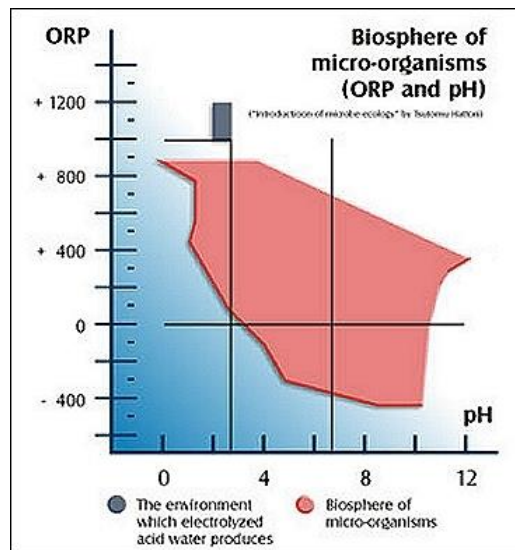
Figure 4. The dependence between acidity and basicity (pH) of NaCl solution and the ORP on the biosphere of micro-organisms.
