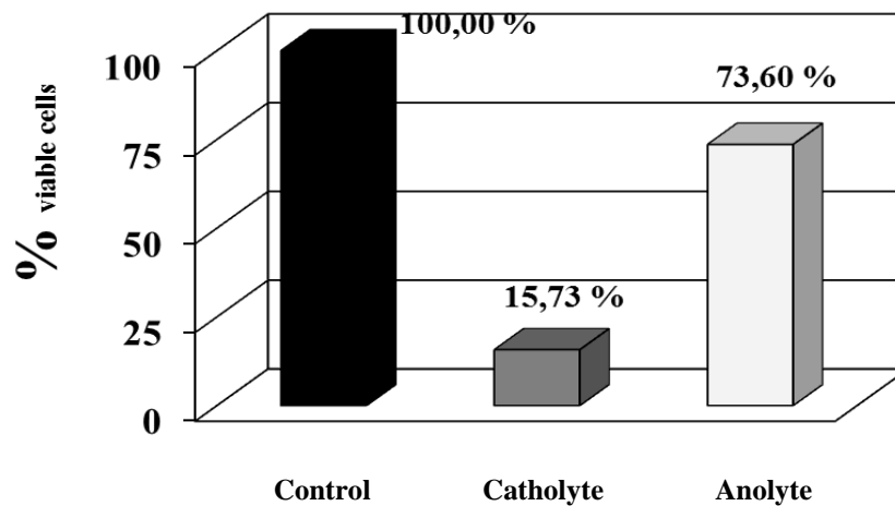
Figure 3. Percentage of viable cells of E. coli DH5a after the treatment with catholyte and anolyte relative to the non-electroactivated water.
