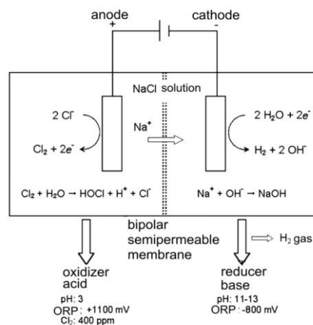
Figure 1. Laboratory setting of diaphragm electrolysis method for the preparation of acid (anolyte) and
