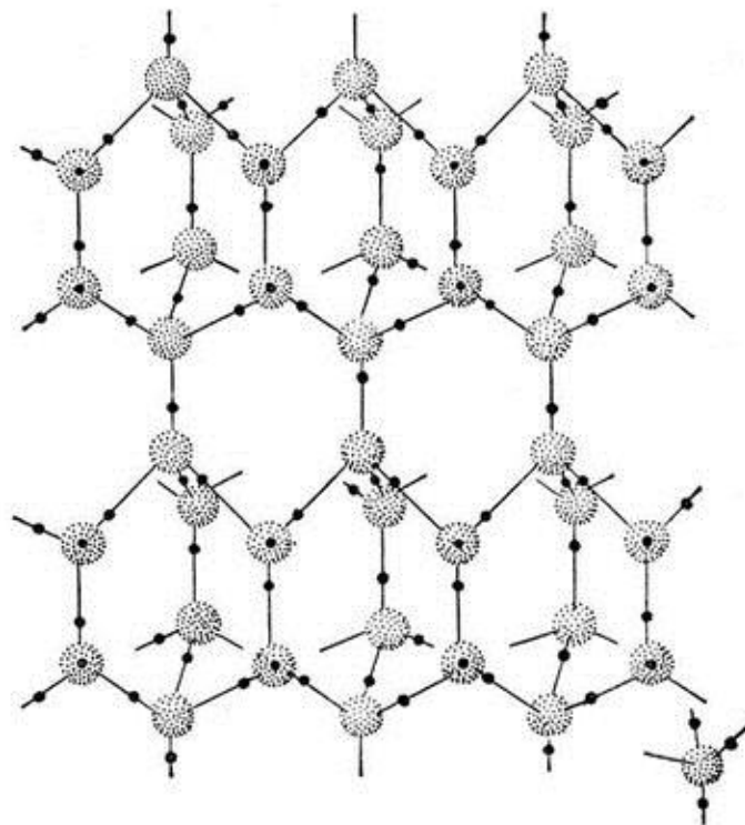
Figure 2. Hydrogen bonding in crystalline structure of natural ice I_h under the temperature -10^{\circ}C and
