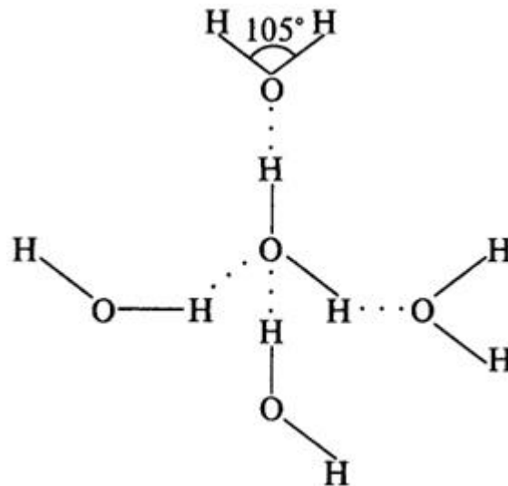
Figure 1. Hydrogen bonding between four individual \text{H}_2\text{O} molecules. It is shown the value of the angle between the covalent \text{H-O-H} bond in \text{H}_2\text{O} molecule.
