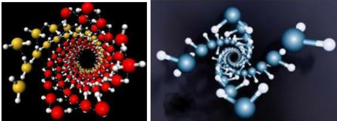
Figure 3. Structures of water crystals in carbon nanotubes according to computer simulations (Bai et al. , 2006) (diameter of nanotubes 1.35–1.90 nm; pressure 10–40000 atm; temperature -23 °C): a) – a general view of the crystal structure of water in nanotubes, b) – the inner wall of the structure of water.
