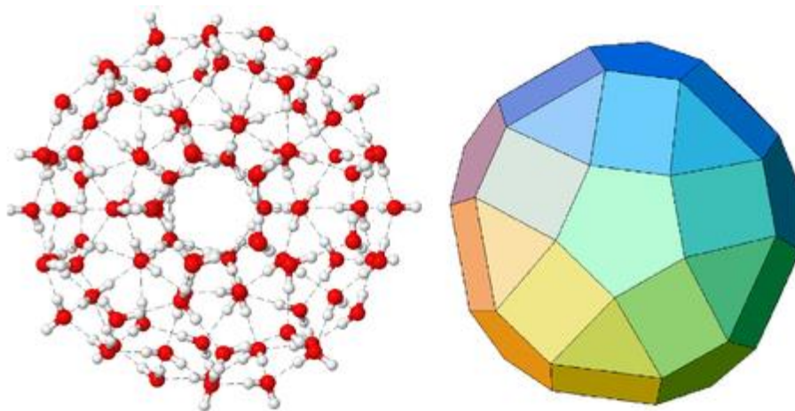
Figure 12. Icosahedron cluster based on 100 H 2 O molecules and the underlying structure according to M. Chaplin’s model.
