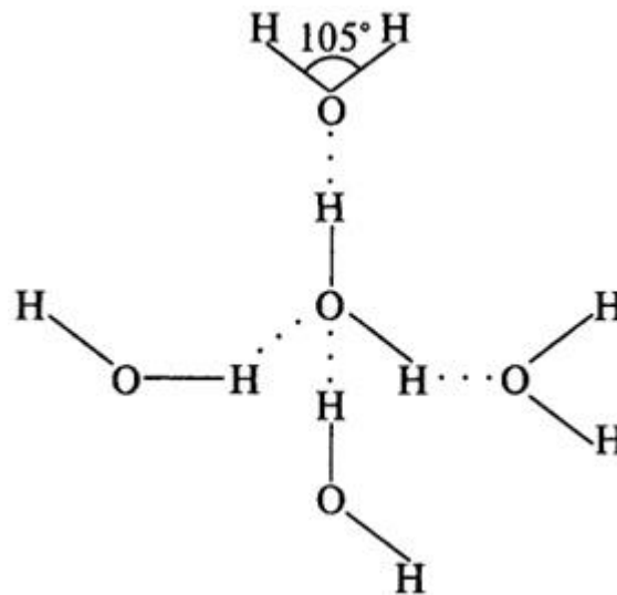
Figure 1. Hydrogen bonding between four individual \text{H}_2\text{O} molecules. It is shown the value of the angle between the covalent \text{H}-\text{O}-\text{H} bond in \text{H}_2\text{O} molecule.
