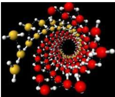
Figure 3. Structures of water crystals in carbon nanotubes according to computer simulations (Bai et al. , 2006) (diameter of nanotubes 1.35–1.90 nm; pressure 10–40000 atm; temperature -23^{\circ}\text{C} ): a) – a general view of the crystal structure of water in nanotubes, b) – the inner wall of the structure of water.
