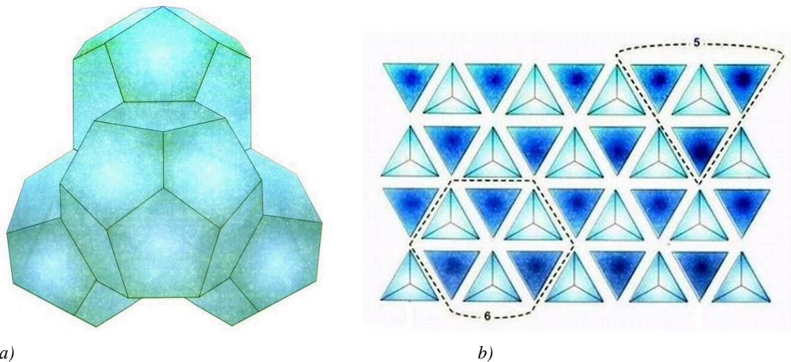
Figure 11. Model of water associates according to S.V. Zenin: a) – associate of 57 H 2 O molecules, tetrahedron of four dodecahedron (“quantum”); b) – bulk packaging of "quanta" (Zenin, 1999).
