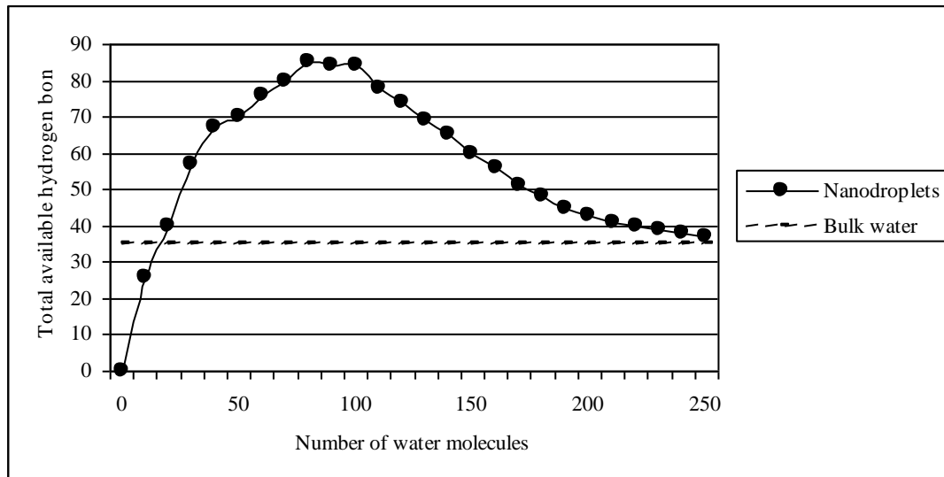
Figure 6. The total number of hydrogen bonds depending on the number of water molecules in clusters.
