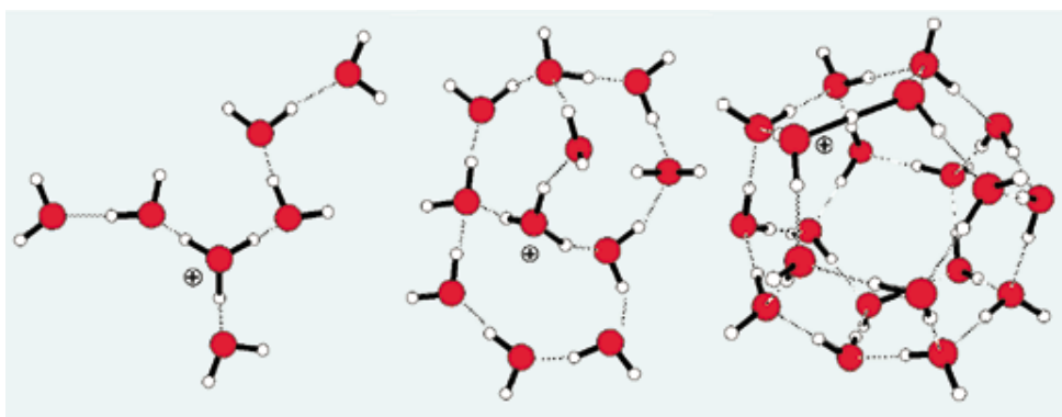
Figure 13. Formation of ionic clusters (\text{H}_2\text{O})_{20}\text{H}_3\text{O}^+ or (\text{H}_2\text{O})_{21}\text{H}^+ with captured hydronium ion \text{H}_3\text{O}^+ .
