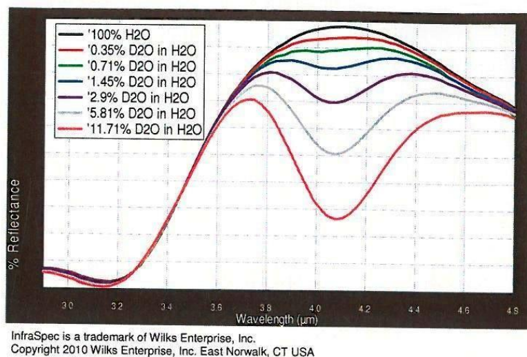
Figure 14. The typical IR-spectra of water with varying content of deuterium
