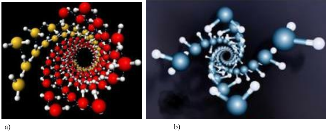
Figure 3. Structures of water crystals in carbon nanotubes according to computer simulations (Bai et al. , 2006) (diameter of nanotubes 1.35–1.90 nm; pressure 10–40000 atm; temperature -23 °C): a) – a general view of the crystal structure of water in nanotubes, b) – the inner wall of the structure of water.
