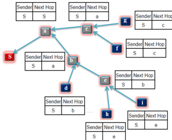
Figure 2: Join-Table propagation
