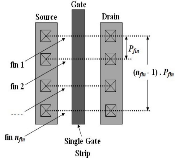
Figure 2: SG-mode FinFET
