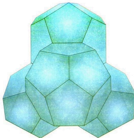
Figure 12. Model of water associate from 57 \text{H}_2\text{O} molecules. Tetrahedron of four dodecahedron
