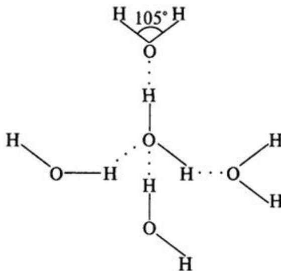
Figure 1. Hydrogen bonding between four individual \text{H}_2\text{O} molecules. It is shown the value of the angle between the covalent H–O–H bond in \text{H}_2\text{O} molecule.
