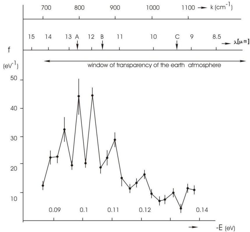
Figure 7. NES-spectrum of deionized water (chemical purity 99.99%, pH = 6.5–7.5, total mineralization 200 mg/l, electric conductivity 10 \mu\text{S}/\text{cm} ). On the horizontal axis shows the energy of the H...O hydrogen bonds in the associates -E (eV). The vertical axis – energy distribution function -f ( \text{eV}^{-1} ). k – the vibration frequency of the H–O–H atoms ( \text{cm}^{-1} ); \lambda – wavelength (mm).
