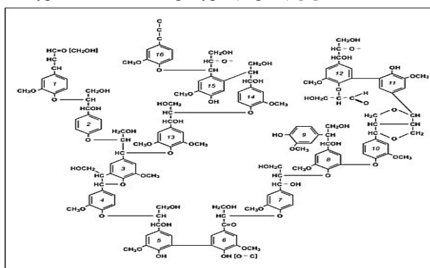
Fig. 3. A structural model of softwood lignin [8]
