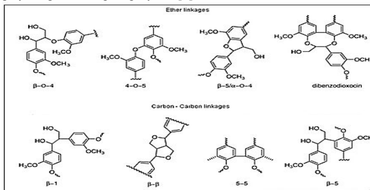
Fig. 2. Common inter monomeric linkages in a lignin molecule
