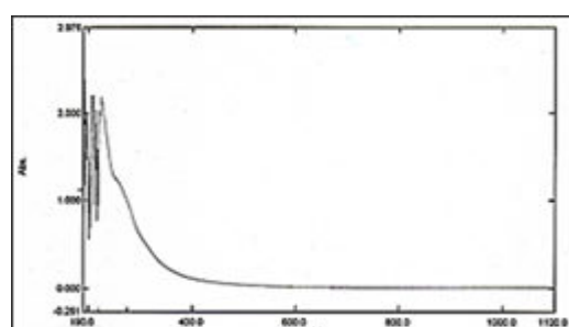
Fig. 13. UV-Vis. Spectrum of Phoenix – JAMAL AL-DEEN pruning lignin.
