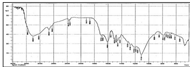
Fig. 4. FT – IR Spectrum of Phoenix – MAKTOM pruning lignin.
