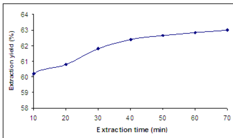
Figure 3. Effect of extraction time on extraction yield (Temperature = 80°C; Ratio of water to raw material = 200).
