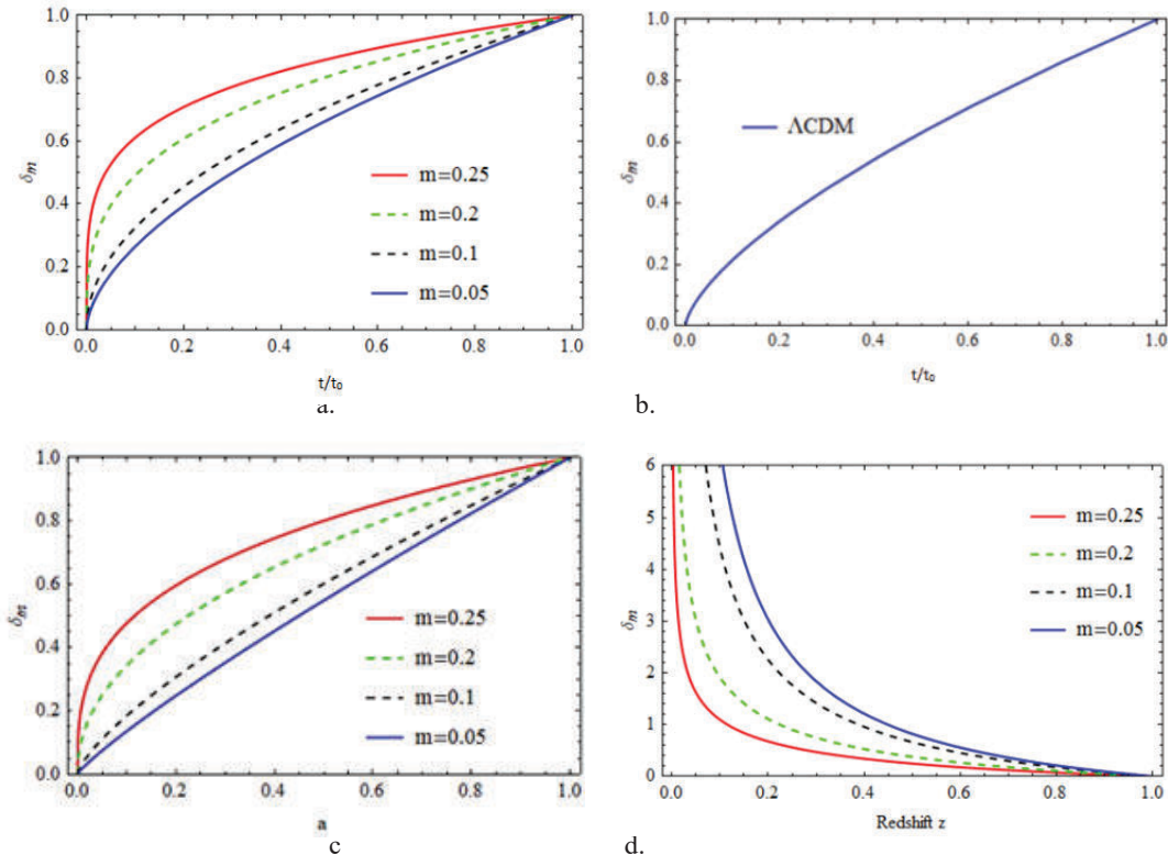
Figure2. Graphs with different values of m , they are compared to that in the \Lambda CDM standard cosmological model.
