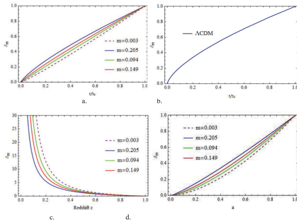
Figure1. Graphs with different values of m ,
