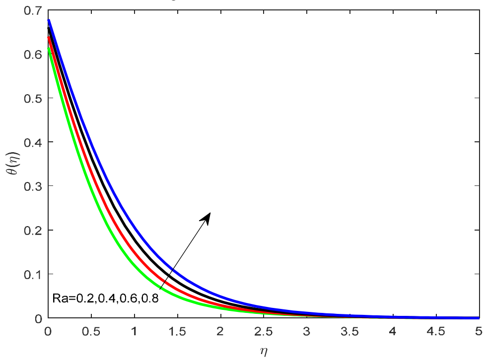
Fig.6 Effect of Ra on thermal field
