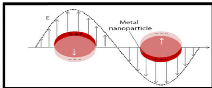
Figure 1. Schematic illustration of a non-propagating localized surface plasmon.
