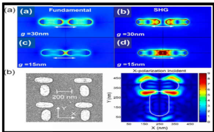
Figure 5. SHG from coupled nanoparticles: (a) gold nanoantennas and (b) gold T-dimers. Panel (a) (adopted from ref. 121). Panel (b) (adopted from ref. 153).
