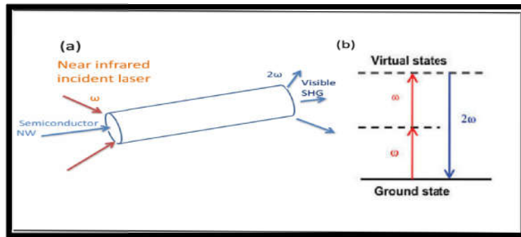
Figure 3. (a) Diagram of the SHG mechanism in semiconductor nanowire. (b) Energy-level diagram describing second-harmonic generation.
