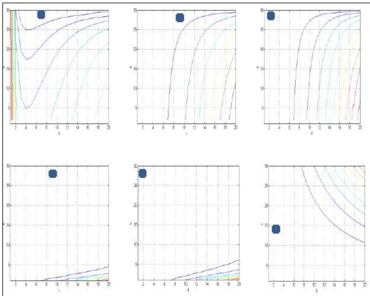
Figure 5. Six 2-parameter combinations of response surfaces for St. Johns River. Up: from left to right (a-b, a-c, and a-d combinations). Down: from left to right (b-c, b-d, and c-d combinations)
