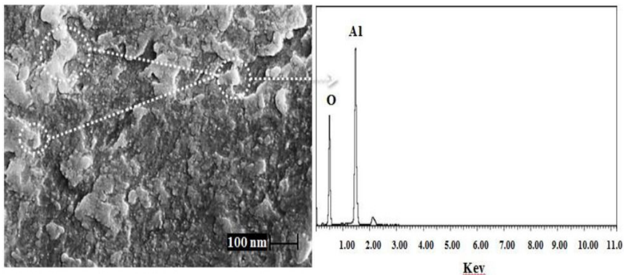
Fig.4. SEM image and EDS plots showing the formation of \text{Al}_2\text{O}_3 oxide on the NiCrAlY grains during milling process.
