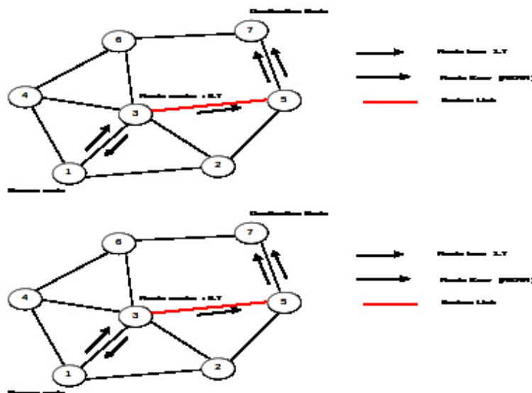
Fig. 4. Route Maintenance in AODV [8]
