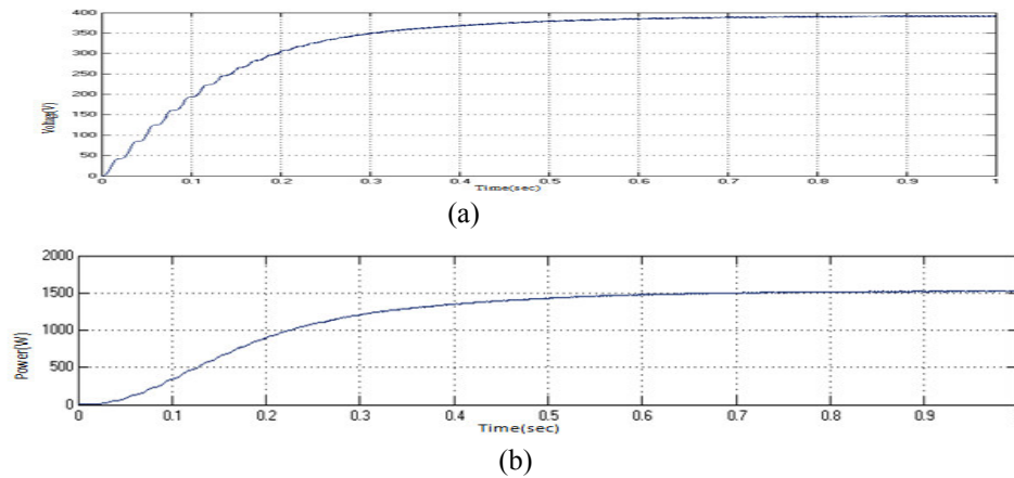
Figure14. PV system with two-model MPPT technique at 1000W/m 2 irradiation (a) Voltage (b) Power The output voltage and power of a PV system using two-model MPPT method are shown. At an irradiation of 100W/m 2 , the voltage and power of a PV system are as shown in figure14.
