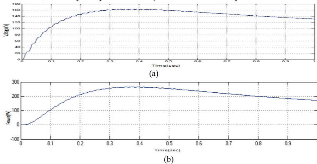
Figure15. PV system with two-model MPPT technique at 600W/m 2 irradiation (a) Voltage (b) Power For an irradiation of 600W/m 2 , the output voltage and power characteristics are as shown in figure15.
