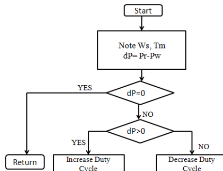
Figure8. MPPT algorithm for WECS
