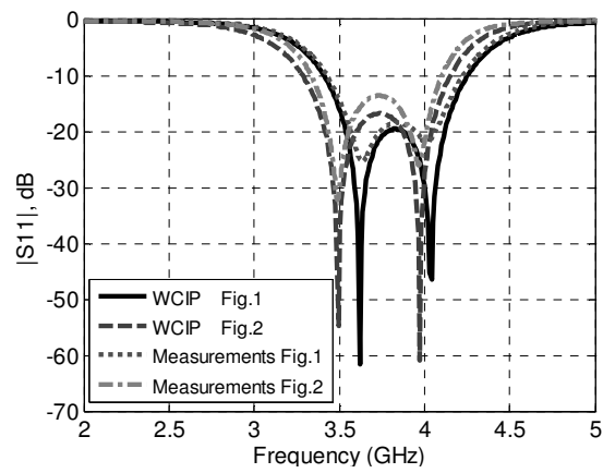
Figure 4. Reflexion parameters ( S_{11} ) of the SINRD filter
