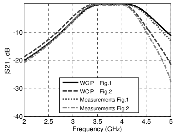
Figure 4. Transmission parameters ( S_{21} ) of the SINRD filter
