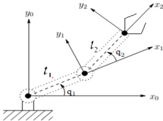
Figure 1 A 2R Planner Robot Manipulator
