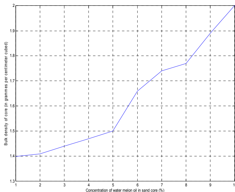
Figure 11:-Bulk density (in \text{g/cm}^3 ) against increasing water melon oil binder content
