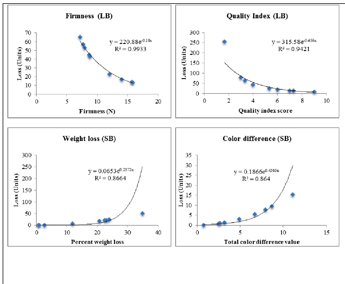
Figure 1. Taguchi quadratic loss functions obtained for all quality attributes. (LB=larger the better, SB=smaller the better)
