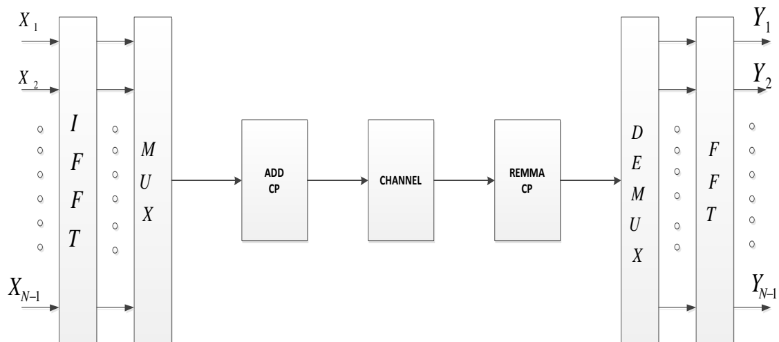
Figure 4: Block Diagram of OFDM System.
