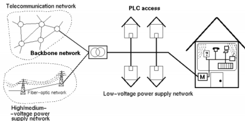
Figure 1: PLC Access Network
