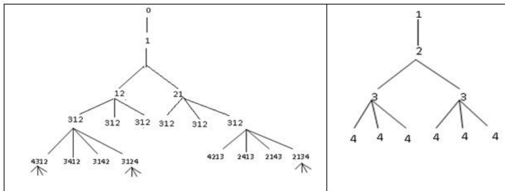
Figure 1. Generating tree of permutation objects according to the object codes (left) and number of children produced (right)
