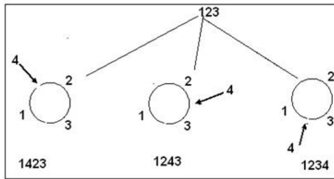
Figure 3. Generating Hamiltonian cycles object using Johnson-Trotter scheme for initial object 123, insertions element 4 gives 3 new objects: 1423, 1243, 1234.
