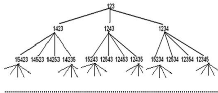
Figure 4. Generating tree of Hamiltonian cycles belong to a complete graph K_n where the nodes are labeled as the object itself started from object with label 123
