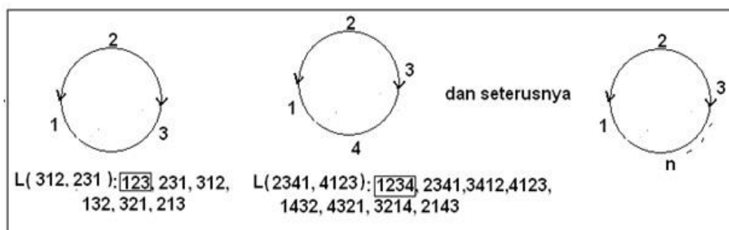
Figure 2. Sets of Labels ( L(\pi, \pi^{-1}) ), for pair of cycle permutations of length n = 3, 4, \dots on a complete graph K_n ,
