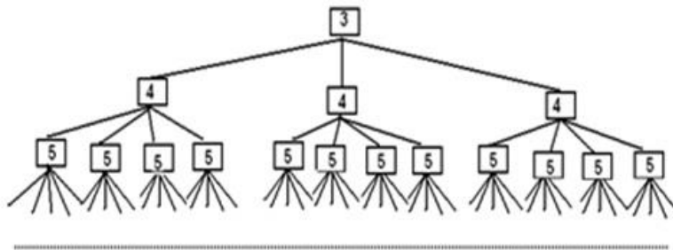
Figure 5. Generating tree of Hamiltonian cycles belong to a complete graph K_n where the nodes are labeled as the number of children nodes started from object of size 3.
