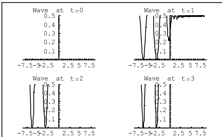
Figure (5) Wave at instants t= 0, 1, 2, 3 .
