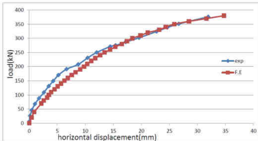
Figure (9): experimental and numerical load-horizontal displacement results of beam A1
