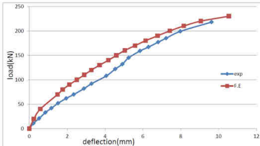
Figure (14): experimental and numerical load-deflection results of beam A45
