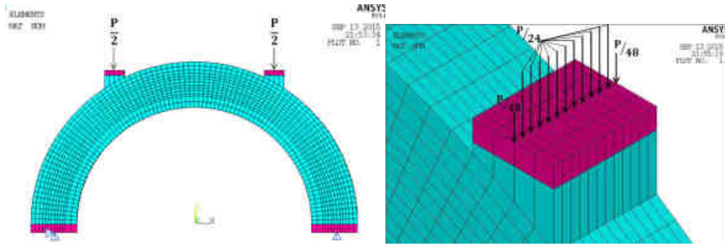
Figure (7): Finite elements mesh and load simulation for beams used in ANSYS program.
