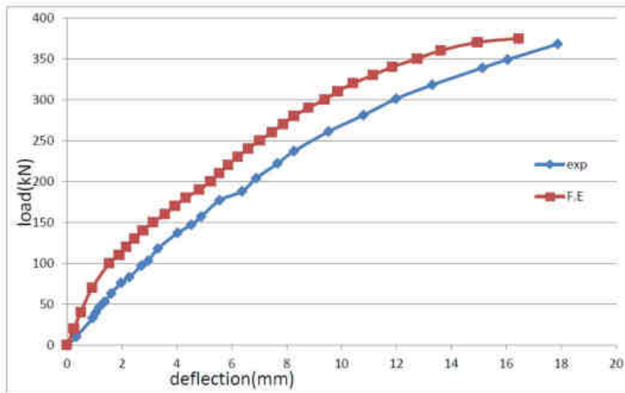
Figure (10): experimental and numerical load-deflection results of beam A90
