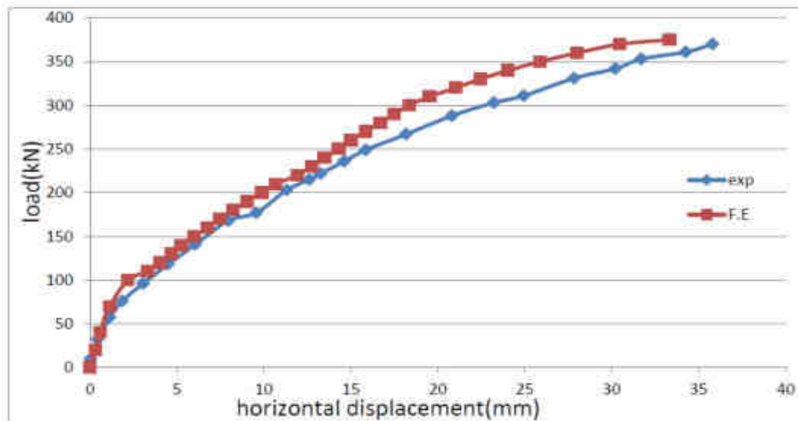
Figure (13): experimental and numerical load-horizontal displacement results of beam A15
