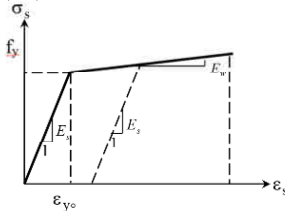
Figure (4): Typical stress-strain curve for steel bar, Mattock (1981)].
