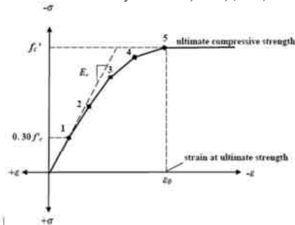
Figure (3): Simplified compressive uniaxial stress-strain curve for concrete Kachlakev et al. (2001).
