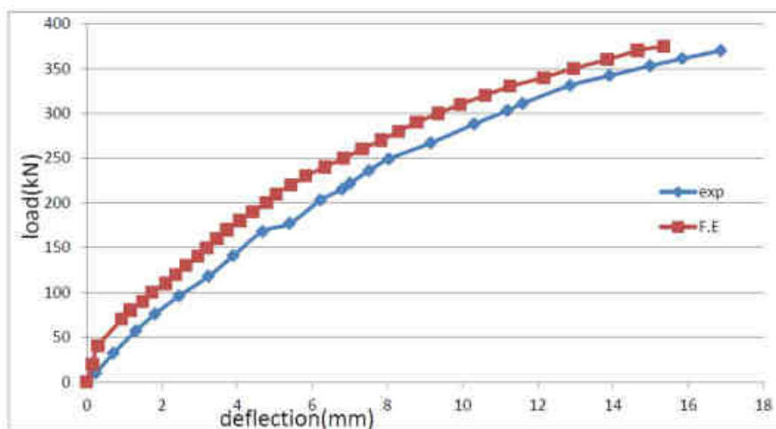
Figure (12): experimental and numerical load-deflection results of beam A15
