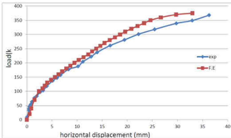
Figure (11): experimental and numerical load-horizontal displacement results of beam A90
