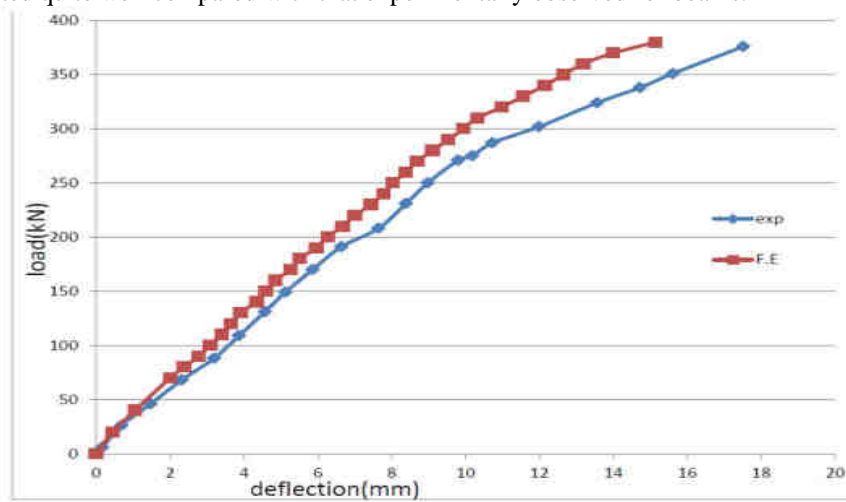
Figure (8): experimental and numerical load-deflection results of beam A1
