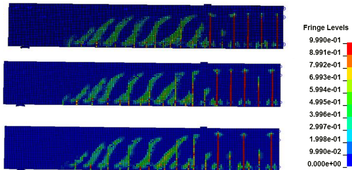
Figure 6. Concrete damage index contours showing the crack patterns at a displacement of 28mm for FE models of RC beam with flange width of (a) 200mm (b) 400mm (c) 600mm (contour represent damage index: 0 = no damage, 1=complete damage)
