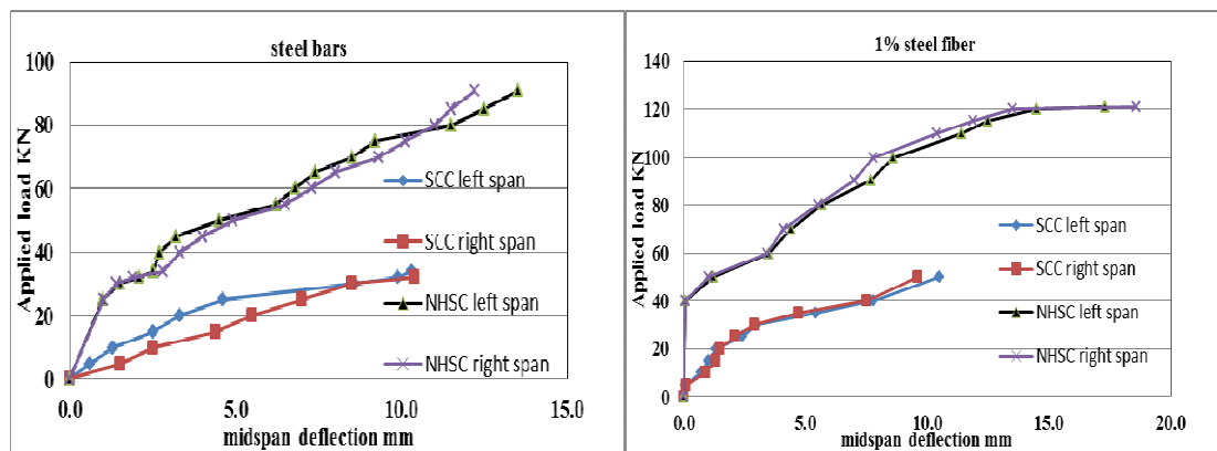
(a) Steel Bar (b) 1% Fiber Reinforcement Figure 9. Comparison of Load-Deflection of the CC and Tested NHSC Slabs
