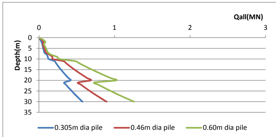
Fig. 5 Chart of allowable pile capacity
