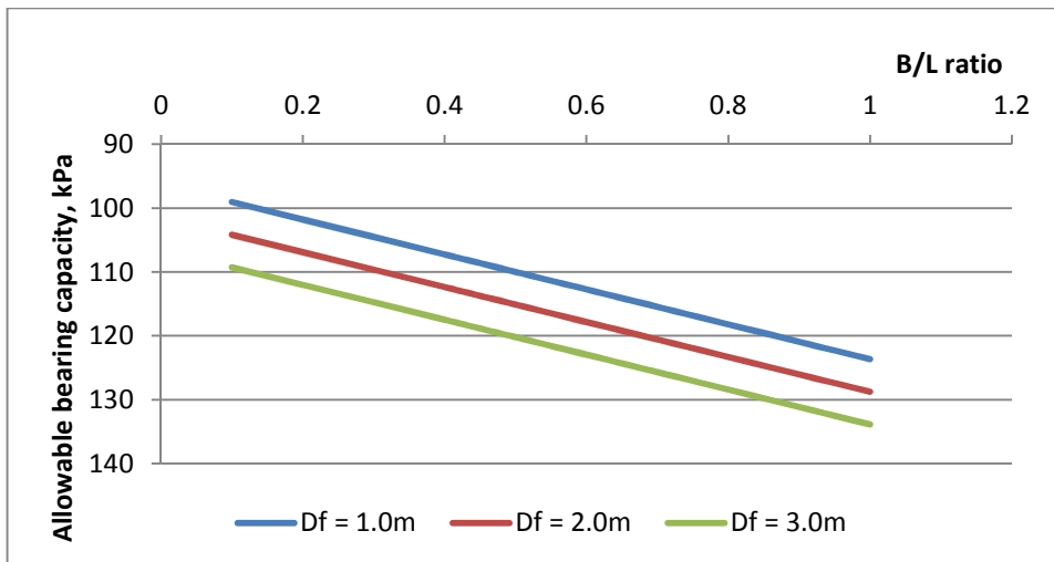
Fig. 3: Chart of allowable bearing capacity
