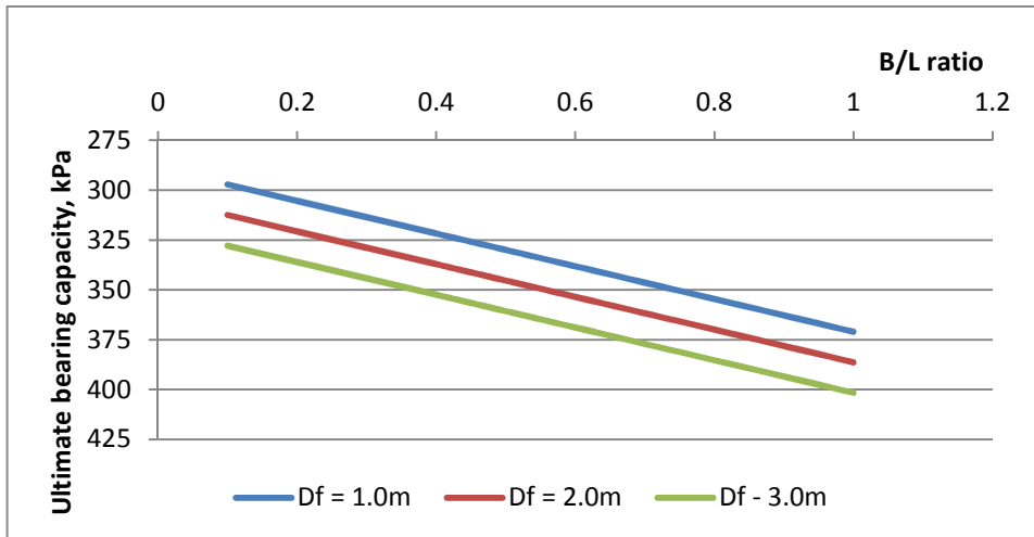
Fig. 2: Chart of ultimate bearing capacity Versus Breadth/Length Ratio
