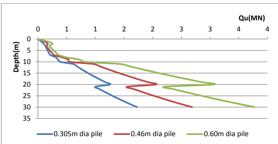
Fig. 4: Chart of ultimate Pile capacity
