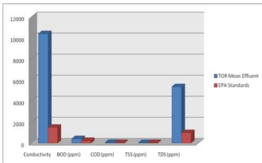
Figure 2: Mean TOR Effluent against the EPA standards
