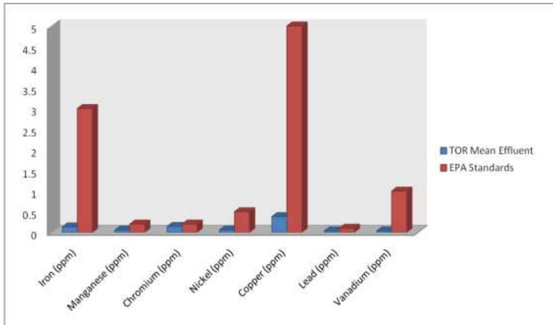
Figure 3: TOR Effluent Heavy metals against EPA standards
