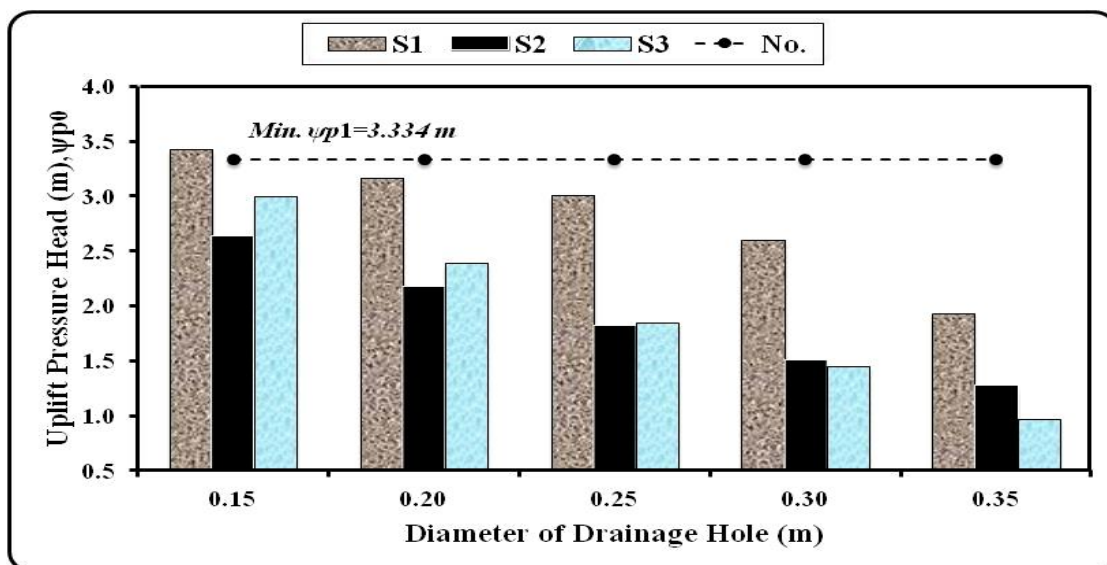
Figure (5): Reduction in uplift pressure head ( \psi_p ) versus drainage hole diameters for different drainage hole types
