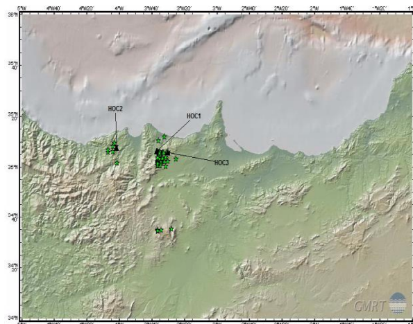
Fig 2: Location map of earthquakes and stations used for this study [14]
