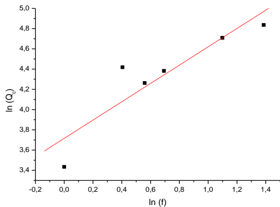
Fig 5. A graph of log(Q) against ln(f) for the AL Hoceima events .
