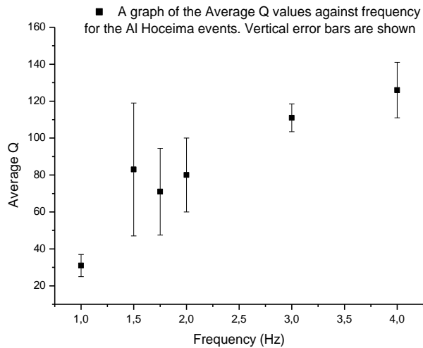
Fig. 4. Shows the distributions of Qc values with frequency for coda window lengths 10 seconds
