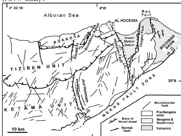
Fig 1. Structural map of the Al Hoceima area and main faults [5]
