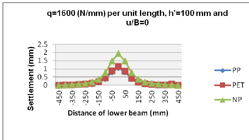
Fig.5 Settlement of lower beam along length for different types of geogrid PP, NP and PET (Test Series-C).
