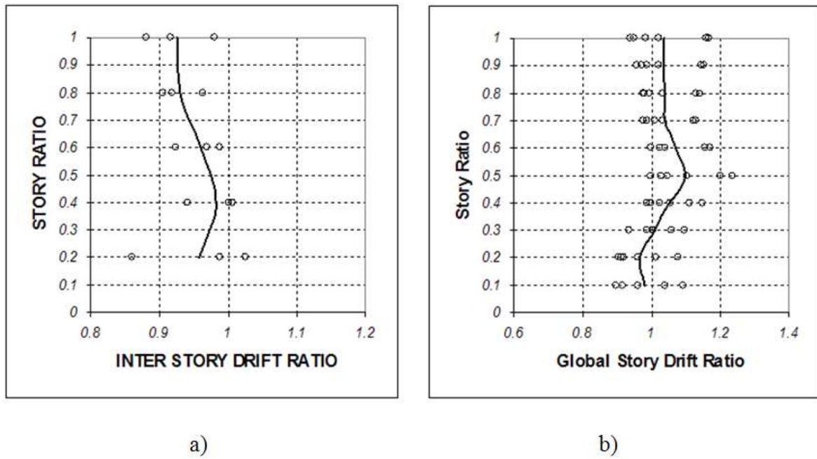
Figure5. Variation diagram, a) ISD, b) GSD for 10-story models.
