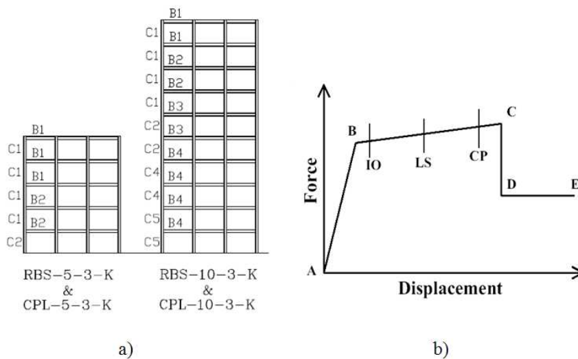
Figure2. a) Designing specifications of analyzed frames under non-linear time history analysis, b) How to define plastic hinges for ductile parts.
