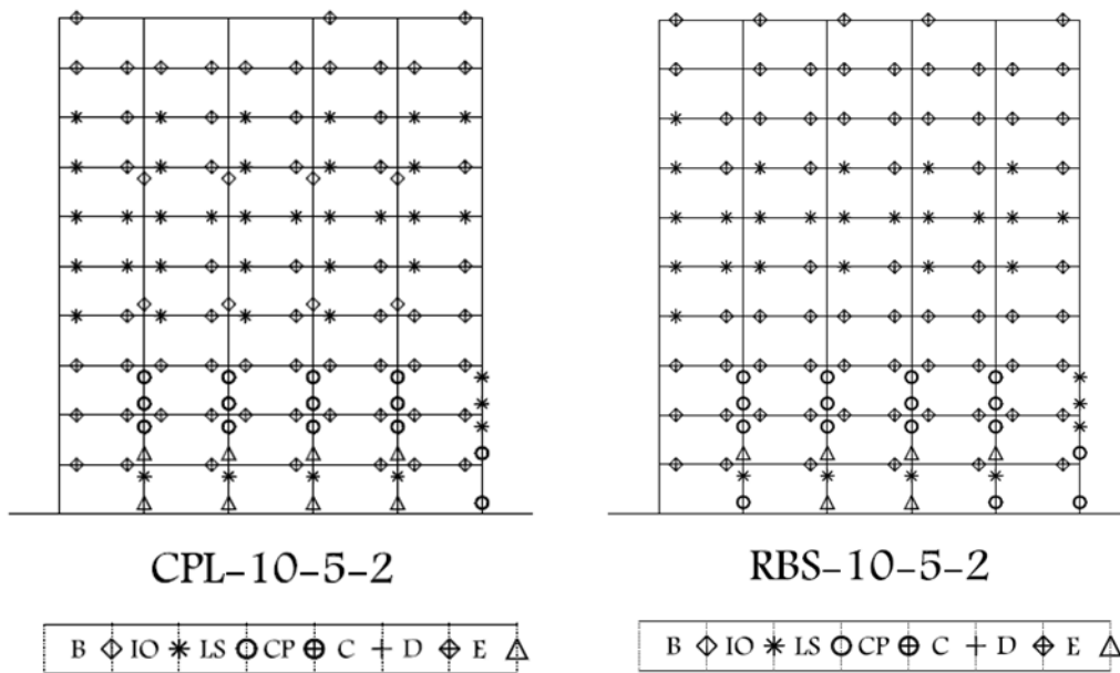
Figure3. The manner of the expansion of plastic hinges in CPL-10-5-2 and RBS-10-5-2 in 9.86 periods (maximum time of displacement on the last story).
