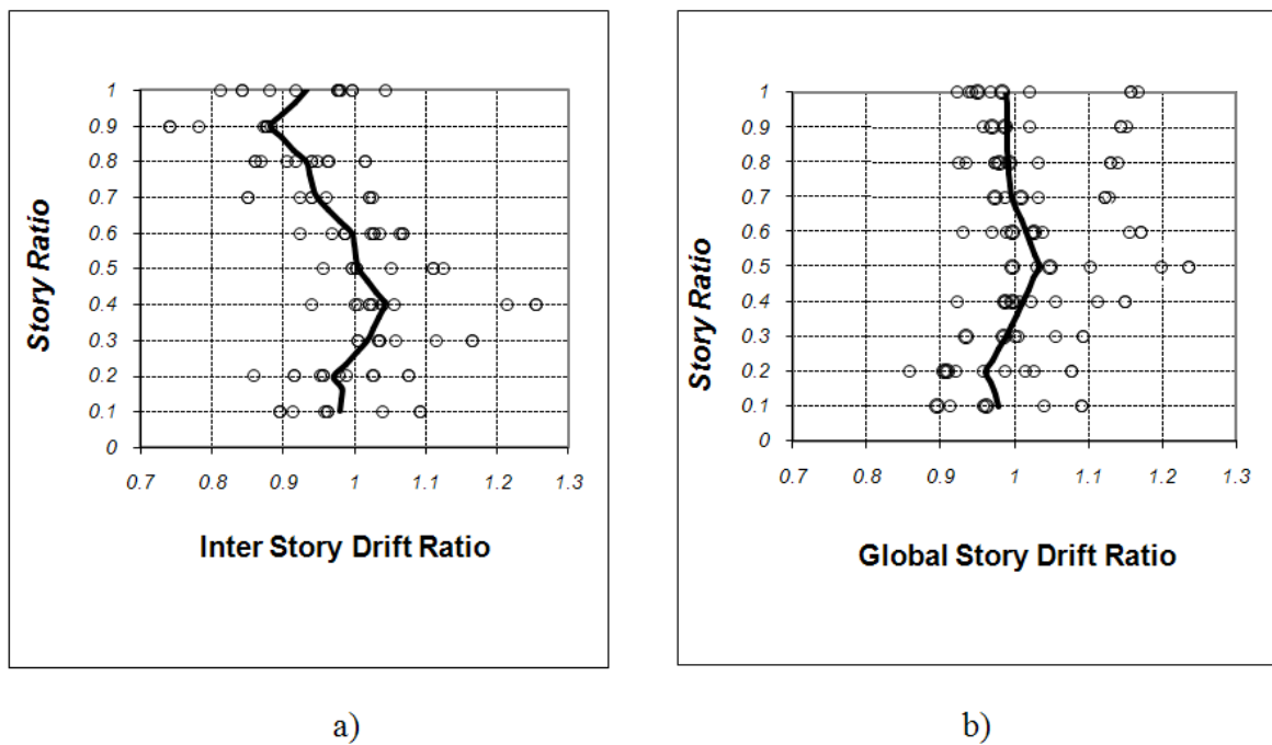
Figure6. Variation diagram, a) ISD, b) GSD for all models.
