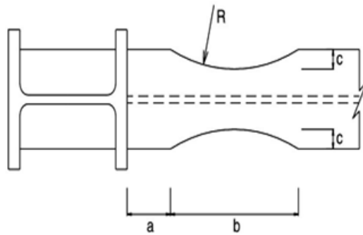
Figure1. Introducing designing parameters in radius cut connection.
