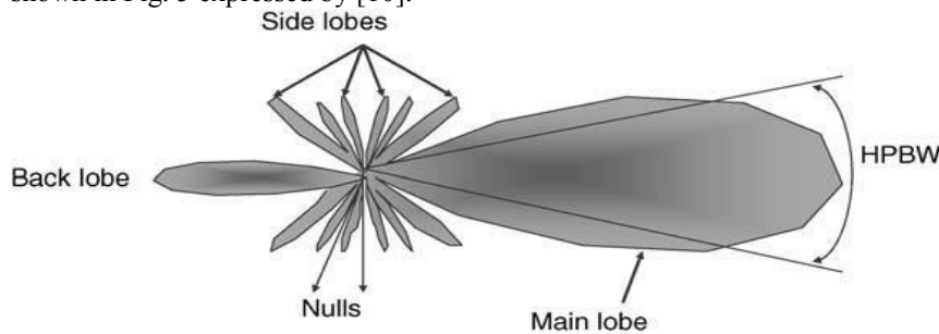
Fig. 5: The Radiation Pattern of an Antenna
