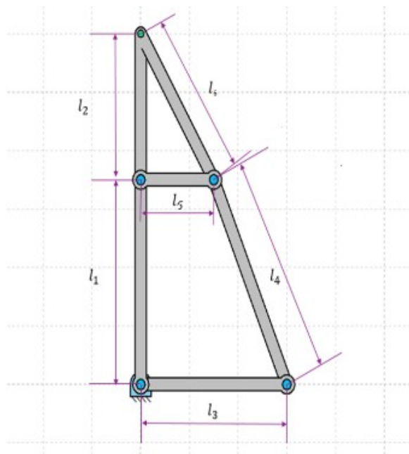
Figure 1. 2-DOF underactuated robotic manipulator
